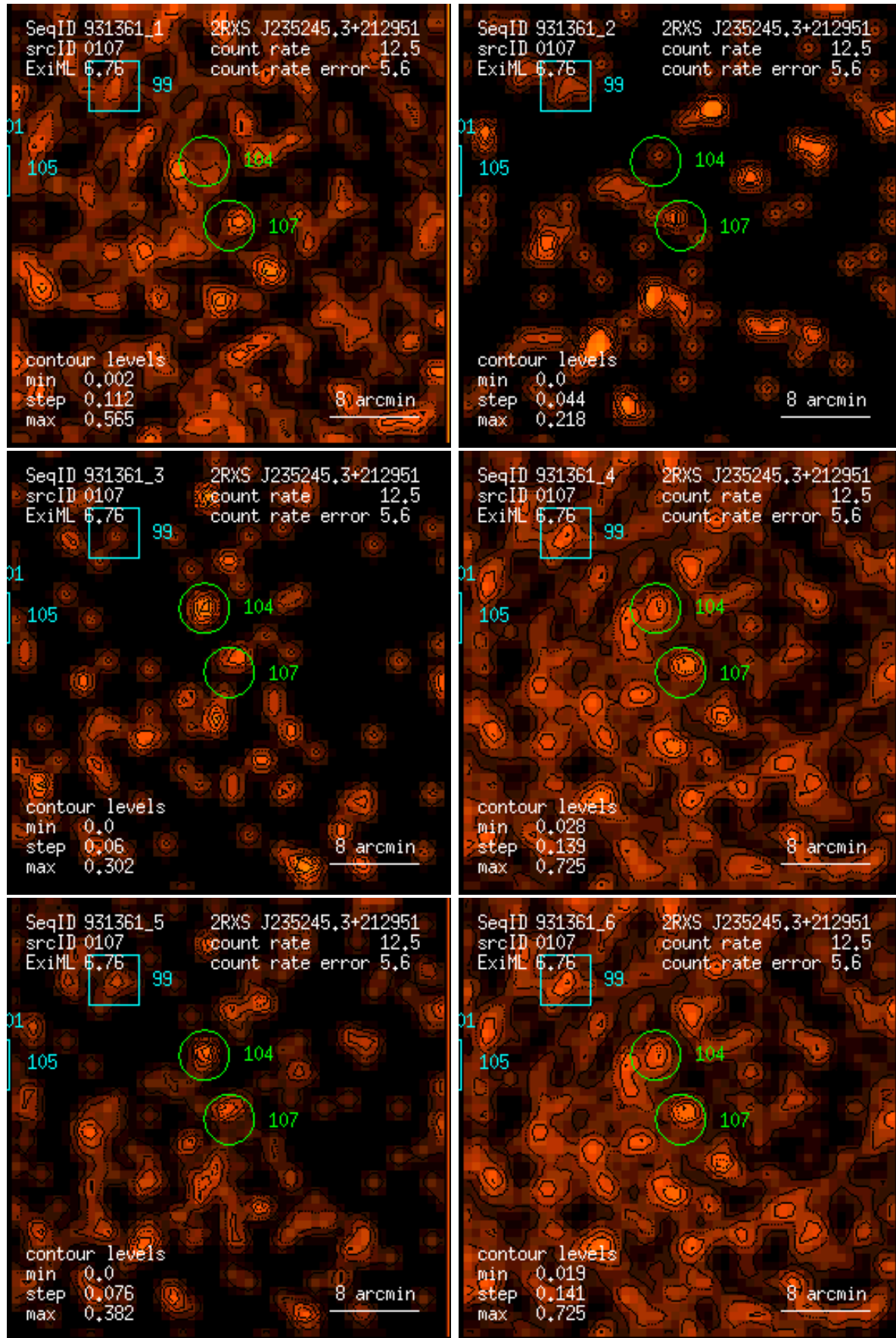
Figure 107: RASS 931361: detection 0107: band rate images, Gaussian filter: (1) PSPC channels 11 – 41, (2) 52 – 90, (3) 91 – 201, (4) 11 – 235, (5) 52 – 201, (6) 11 – 201. Broad band rates in counts/ks. Band rate contour levels in counts/ks/arcmin 2 .
