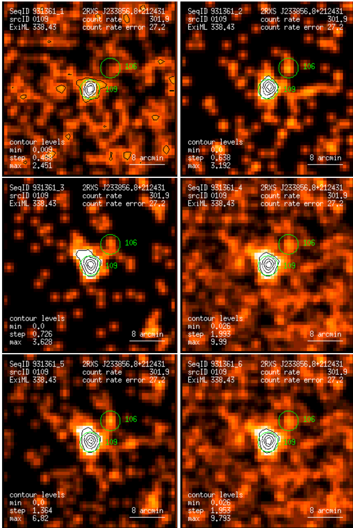
Figure 109: RASS 931361: detection 0109: band rate images, Gaussian filter: (1) PSPC channels 11 – 41, (2) 52 – 90, (3) 91 – 201, (4) 11 – 235, (5) 52 – 201, (6) 11 – 201. Broad band rates in counts/ks. Band rate contour levels in counts/ks/arcmin 2 .
