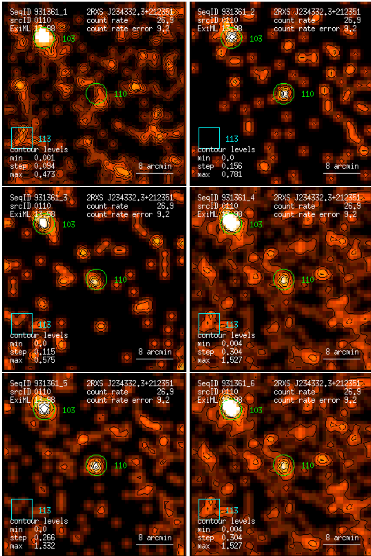
Figure 110: RASS 931361: detection 0110: band rate images, Gaussian filter: (1) PSPC channels 11 – 41, (2) 52 – 90, (3) 91 – 201, (4) 11 – 235, (5) 52 – 201, (6) 11 – 201. Broad band rates in counts/ks. Band rate contour levels in counts/ks/arcmin 2 .
