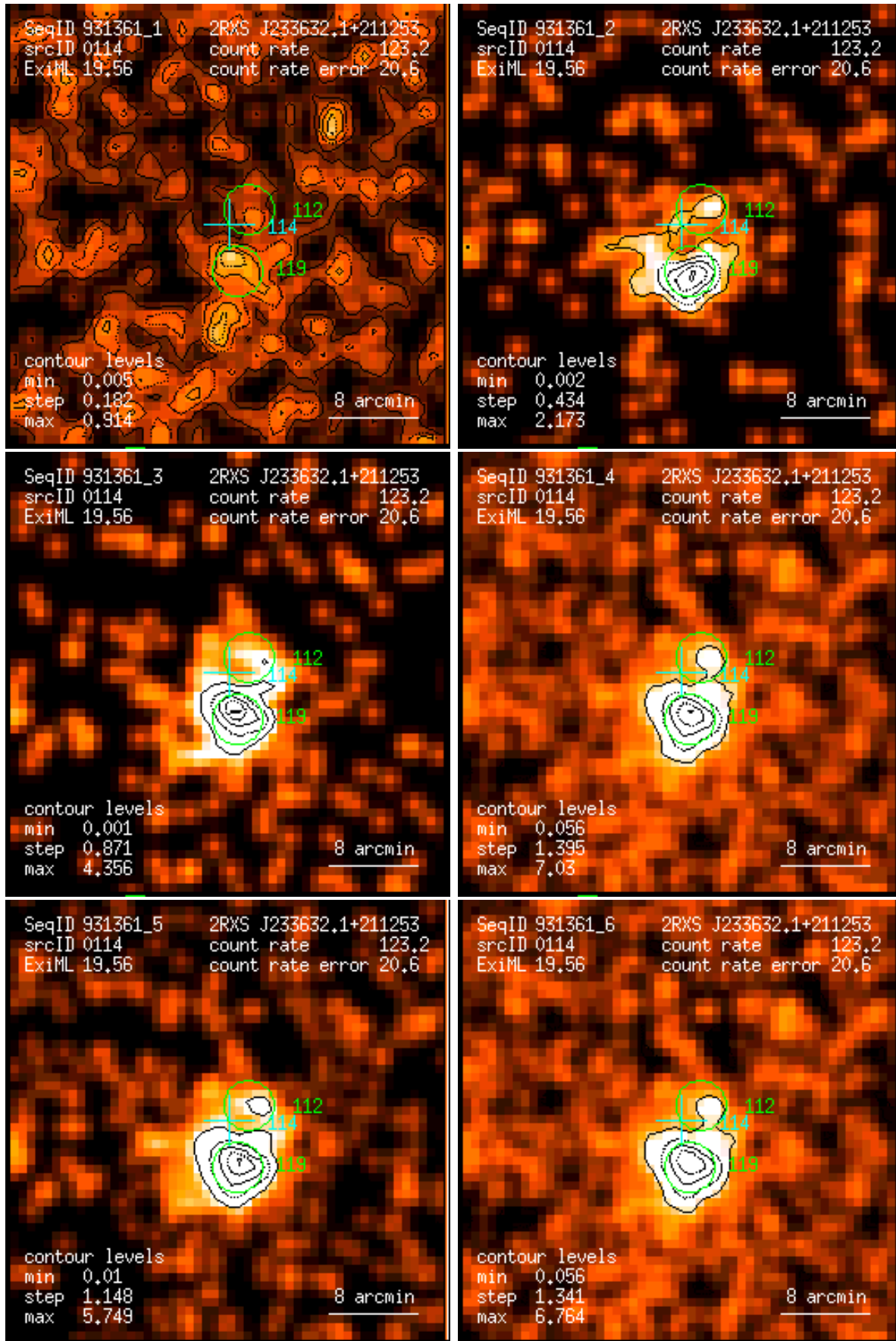
Figure 114: RASS 931361: detection 0114: band rate images, Gaussian filter: (1) PSPC channels 11 – 41, (2) 52 – 90, (3) 91 – 201, (4) 11 – 235, (5) 52 – 201, (6) 11 – 201. Broad band rates in counts/ks. Band rate contour levels in counts/ks/arcmin 2 .
