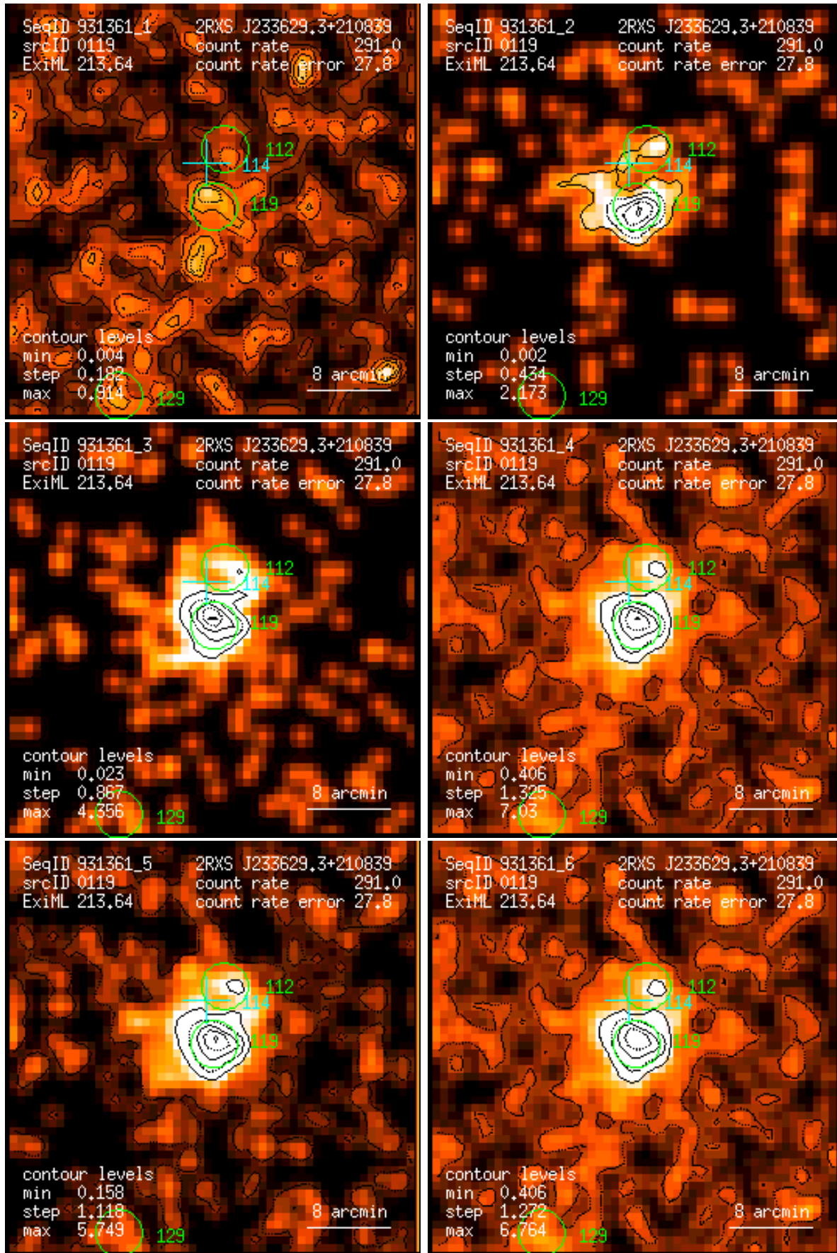
Figure 119: RASS 931361: detection 0119: band rate images, Gaussian filter: (1) PSPC channels 11 – 41, (2) 52 – 90, (3) 91 – 201, (4) 11 – 235, (5) 52 – 201, (6) 11 – 201. Broad band rates in counts/ks. Band rate contour levels in counts/ks/arcmin 2 .
