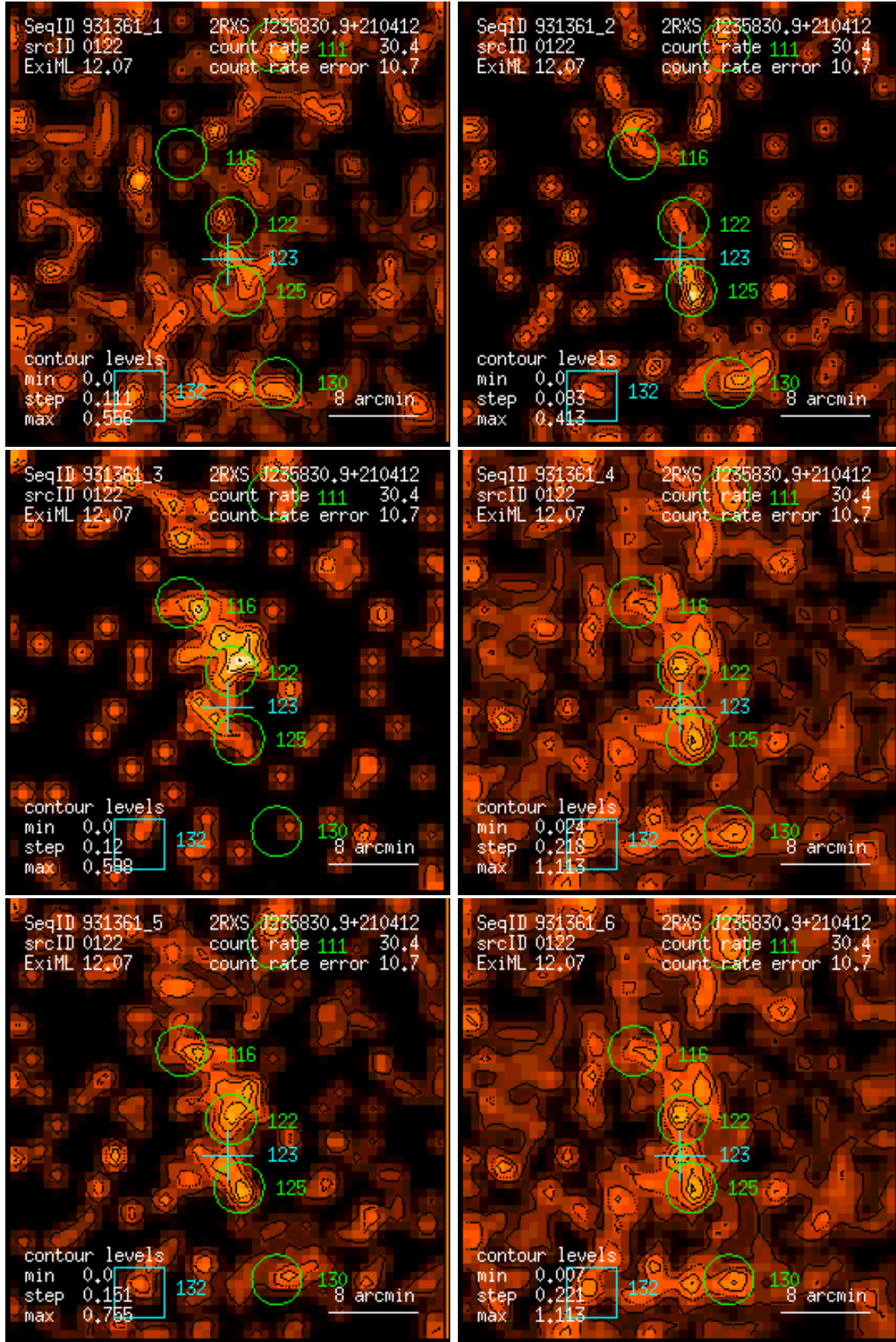
Figure 122: RASS 931361: detection 0122: band rate images, Gaussian filter: (1) PSPC channels 11 – 41, (2) 52 – 90, (3) 91 – 201, (4) 11 – 235, (5) 52 – 201, (6) 11 – 201. Broad band rates in counts/ks. Band rate contour levels in counts/ks/arcmin 2 .
