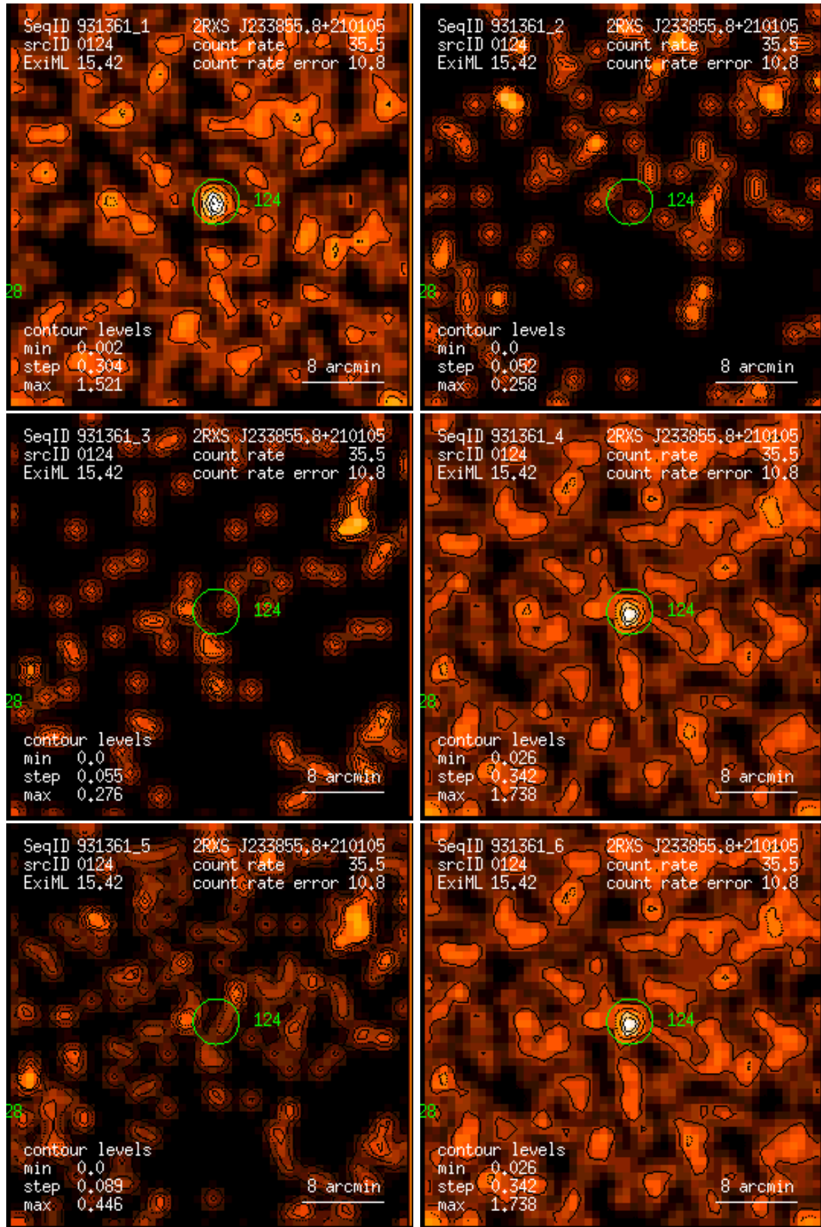
Figure 124: RASS 931361: detection 0124: band rate images, Gaussian filter: (1) PSPC channels 11 – 41, (2) 52 – 90, (3) 91 – 201, (4) 11 – 235, (5) 52 – 201, (6) 11 – 201. Broad band rates in counts/ks. Band rate contour levels in counts/ks/arcmin 2 .
