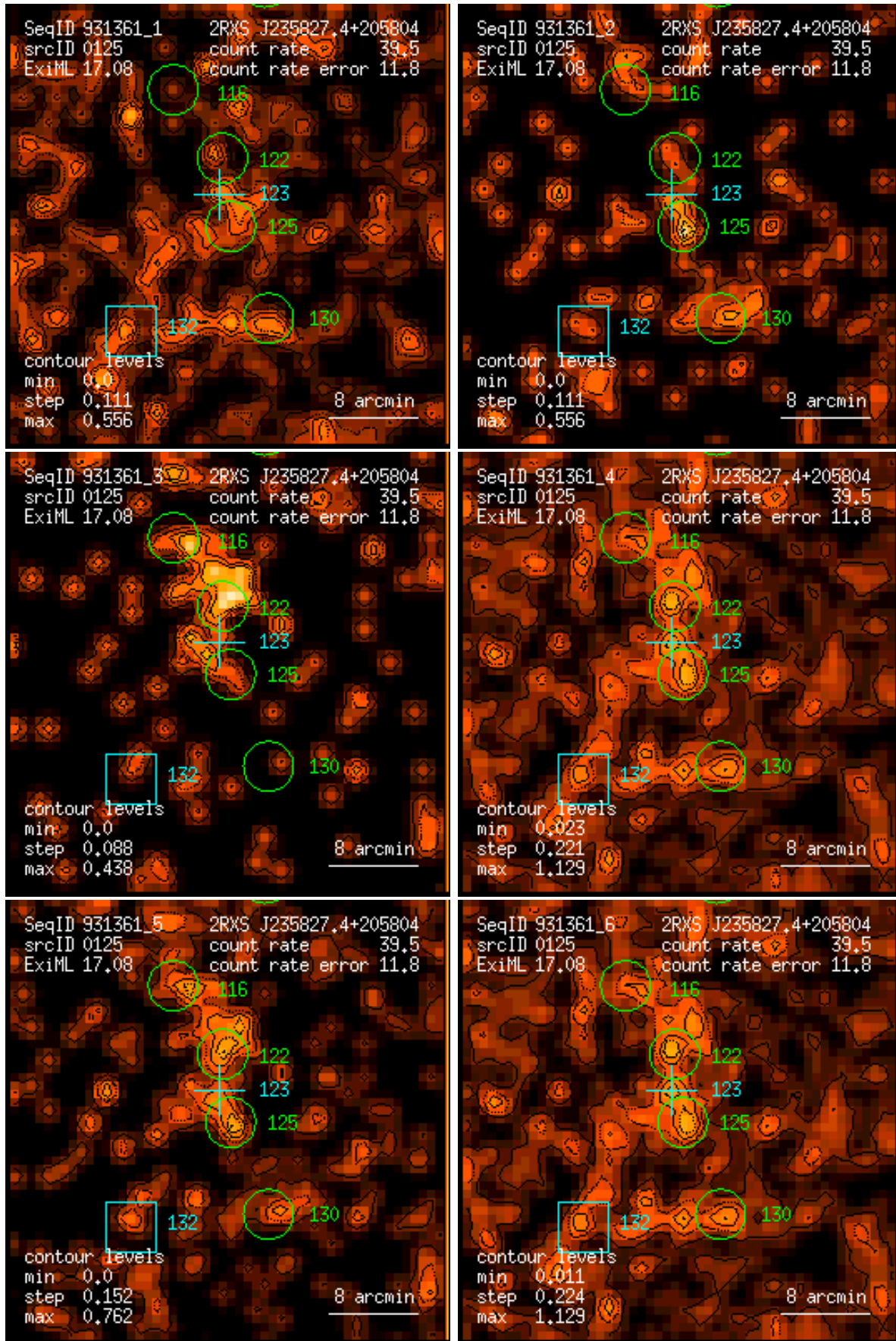
Figure 125: RASS 931361: detection 0125: band rate images, Gaussian filter: (1) PSPC channels 11 – 41, (2) 52 – 90, (3) 91 – 201, (4) 11 – 235, (5) 52 – 201, (6) 11 – 201. Broad band rates in counts/ks. Band rate contour levels in counts/ks/arcmin 2 .
