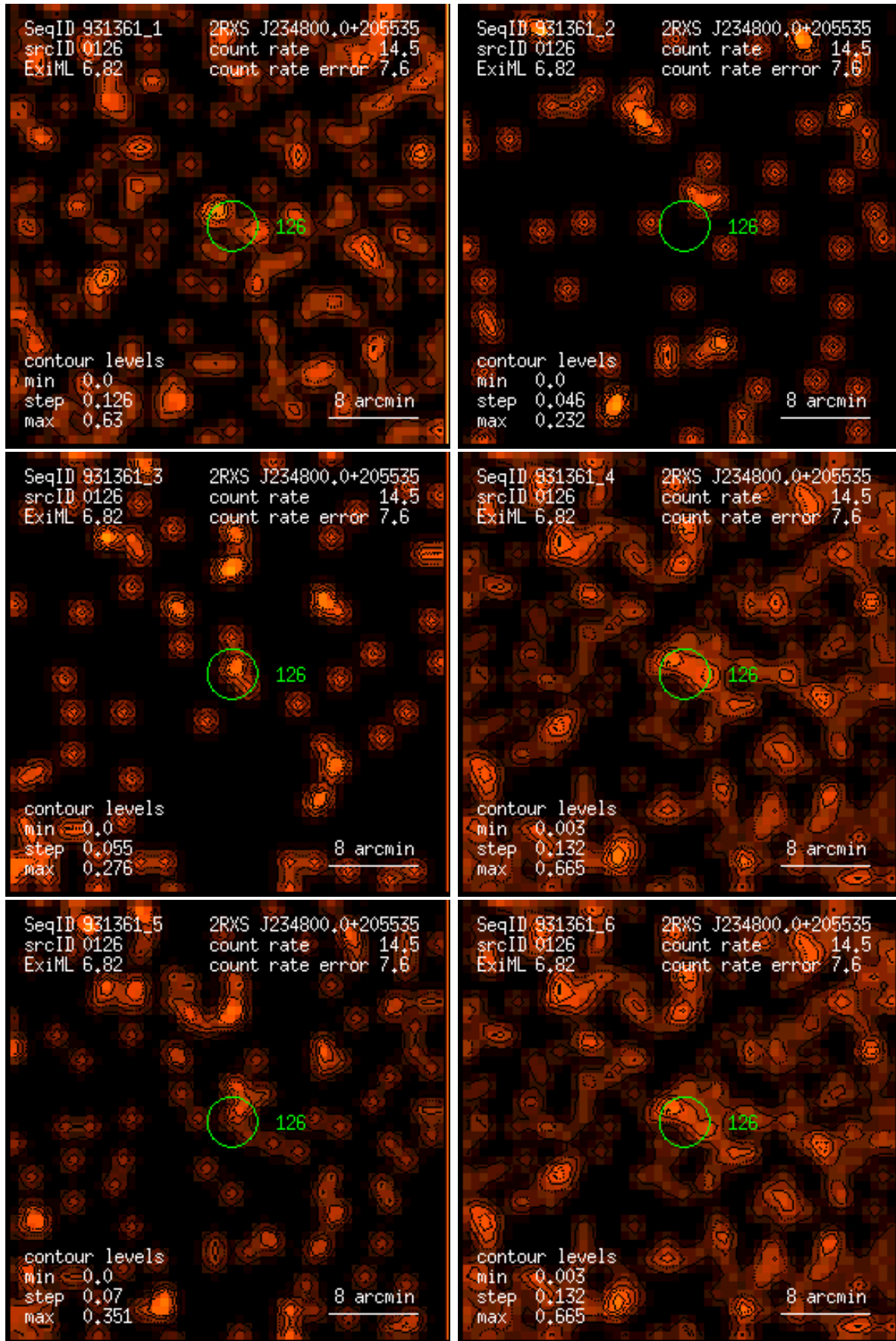
Figure 126: RASS 931361: detection 0126: band rate images, Gaussian filter: (1) PSPC channels 11 – 41, (2) 52 – 90, (3) 91 – 201, (4) 11 – 235, (5) 52 – 201, (6) 11 – 201. Broad band rates in counts/ks. Band rate contour levels in counts/ks/arcmin 2 .
