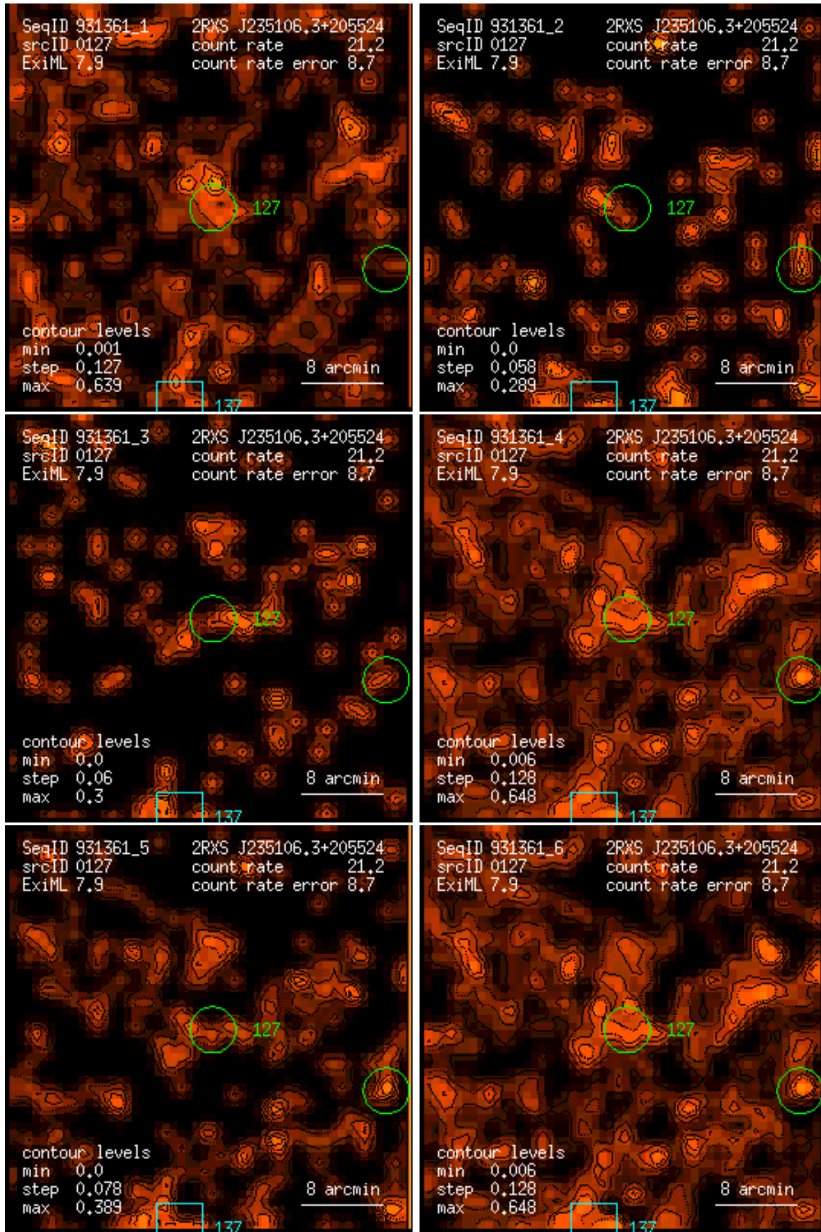
Figure 127: RASS 931361: detection 0127: band rate images, Gaussian filter: (1) PSPC channels 11 – 41, (2) 52 – 90, (3) 91 – 201, (4) 11 – 235, (5) 52 – 201, (6) 11 – 201. Broad band rates in counts/ks. Band rate contour levels in counts/ks/arcmin 2 .
