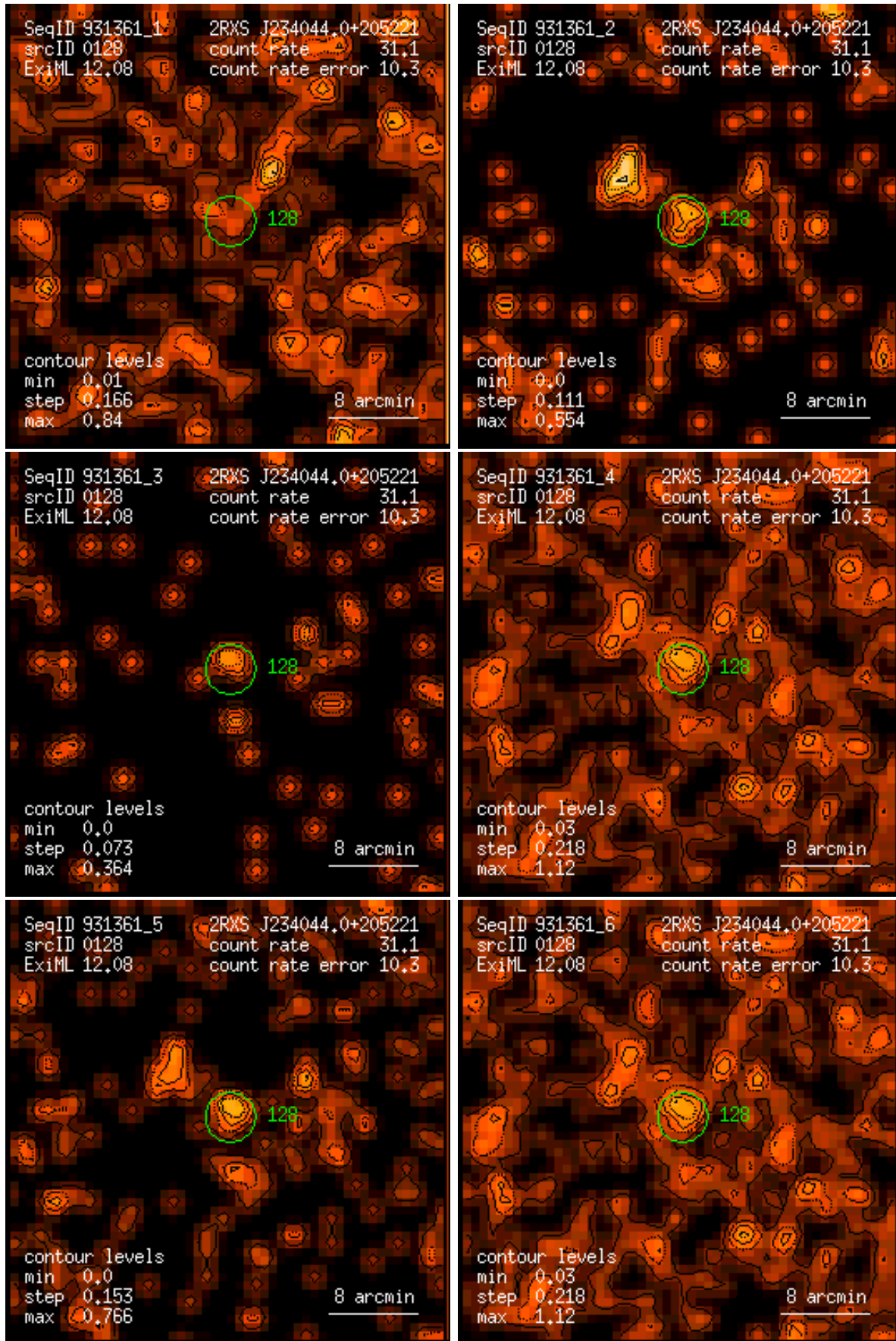
Figure 128: RASS 931361: detection 0128: band rate images, Gaussian filter: (1) PSPC channels 11 – 41, (2) 52 – 90, (3) 91 – 201, (4) 11 – 235, (5) 52 – 201, (6) 11 – 201. Broad band rates in counts/ks. Band rate contour levels in counts/ks/arcmin 2 .
