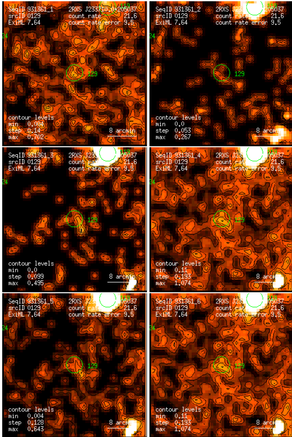
Figure 129: RASS 931361: detection 0129: band rate images, Gaussian filter: (1) PSPC channels 11 – 41, (2) 52 – 90, (3) 91 – 201, (4) 11 – 235, (5) 52 – 201, (6) 11 – 201. Broad band rates in counts/ks. Band rate contour levels in counts/ks/arcmin 2 .
