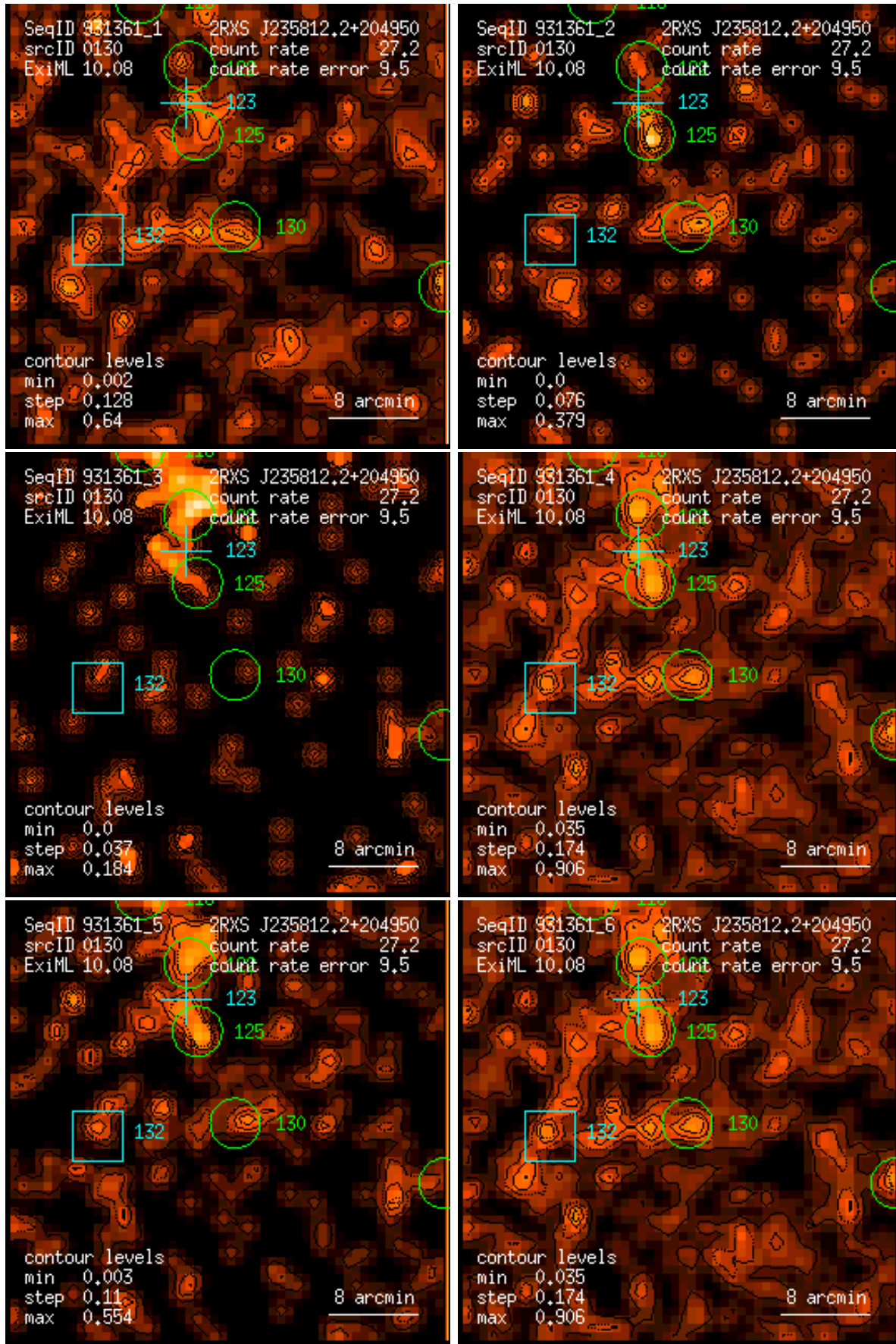
Figure 130: RASS 931361: detection 0130: band rate images, Gaussian filter: (1) PSPC channels 11 – 41, (2) 52 – 90, (3) 91 – 201, (4) 11 – 235, (5) 52 – 201, (6) 11 – 201. Broad band rates in counts/ks. Band rate contour levels in counts/ks/arcmin 2 .
