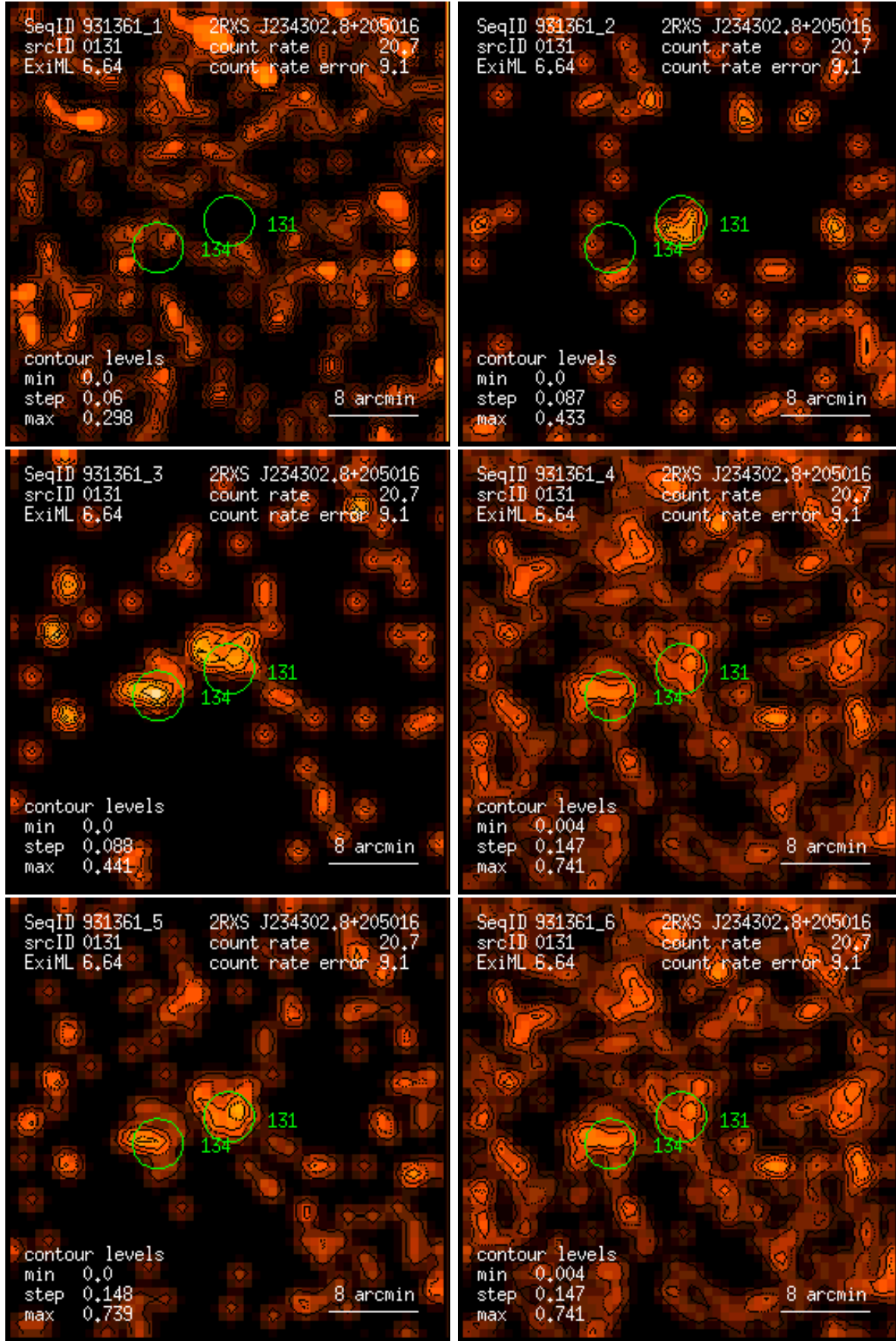
Figure 131: RASS 931361: detection 0131: band rate images, Gaussian filter: (1) PSPC channels 11 – 41, (2) 52 – 90, (3) 91 – 201, (4) 11 – 235, (5) 52 – 201, (6) 11 – 201. Broad band rates in counts/ks. Band rate contour levels in counts/ks/arcmin 2 .
