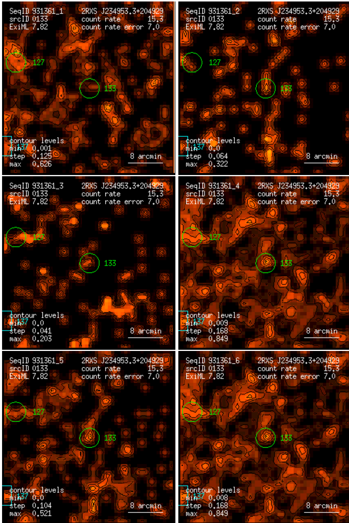
Figure 133: RASS 931361: detection 0133: band rate images, Gaussian filter: (1) PSPC channels 11 – 41, (2) 52 – 90, (3) 91 – 201, (4) 11 – 235, (5) 52 – 201, (6) 11 – 201. Broad band rates in counts/ks. Band rate contour levels in counts/ks/arcmin 2 .
