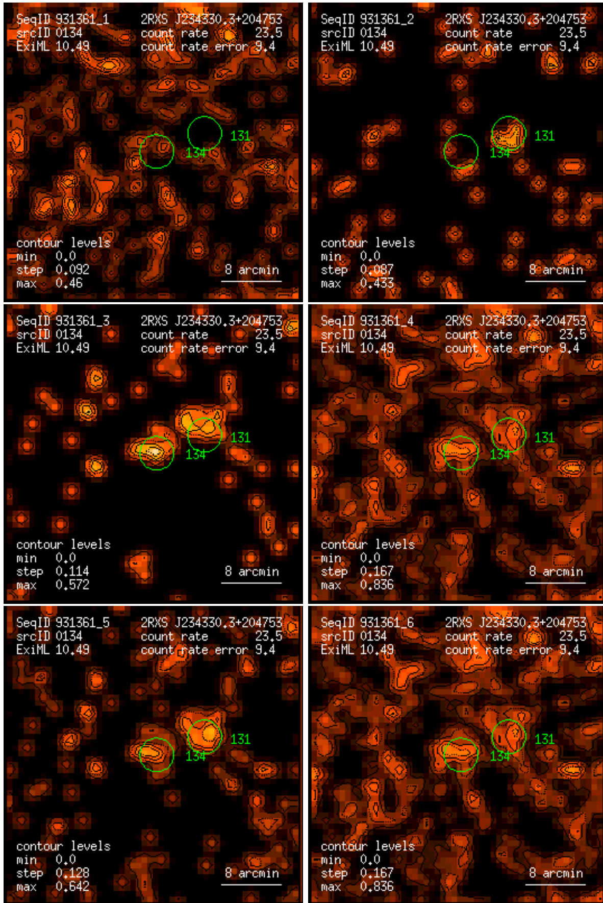
Figure 134: RASS 931361: detection 0134: band rate images, Gaussian filter: (1) PSPC channels 11 – 41, (2) 52 – 90, (3) 91 – 201, (4) 11 – 235, (5) 52 – 201, (6) 11 – 201. Broad band rates in counts/ks. Band rate contour levels in counts/ks/arcmin 2 .
