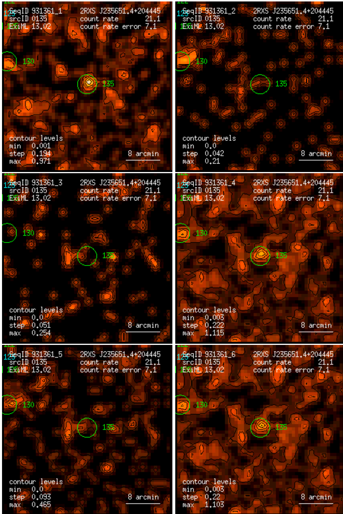
Figure 135: RASS 931361: detection 0135: band rate images, Gaussian filter: (1) PSPC channels 11 – 41, (2) 52 – 90, (3) 91 – 201, (4) 11 – 235, (5) 52 – 201, (6) 11 – 201. Broad band rates in counts/ks. Band rate contour levels in counts/ks/arcmin 2 .
