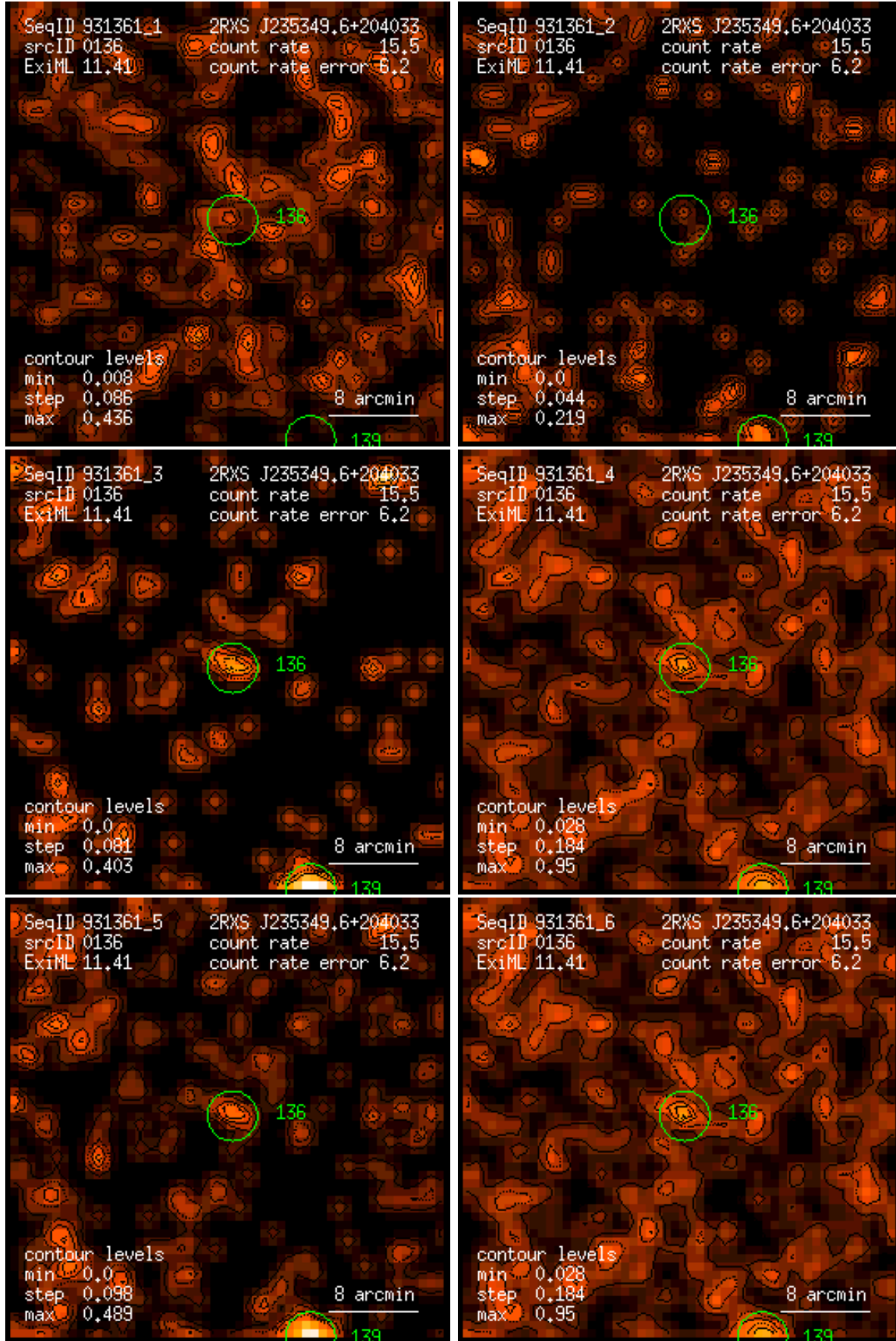
Figure 136: RASS 931361: detection 0136: band rate images, Gaussian filter: (1) PSPC channels 11 – 41, (2) 52 – 90, (3) 91 – 201, (4) 11 – 235, (5) 52 – 201, (6) 11 – 201. Broad band rates in counts/ks. Band rate contour levels in counts/ks/arcmin 2 .
