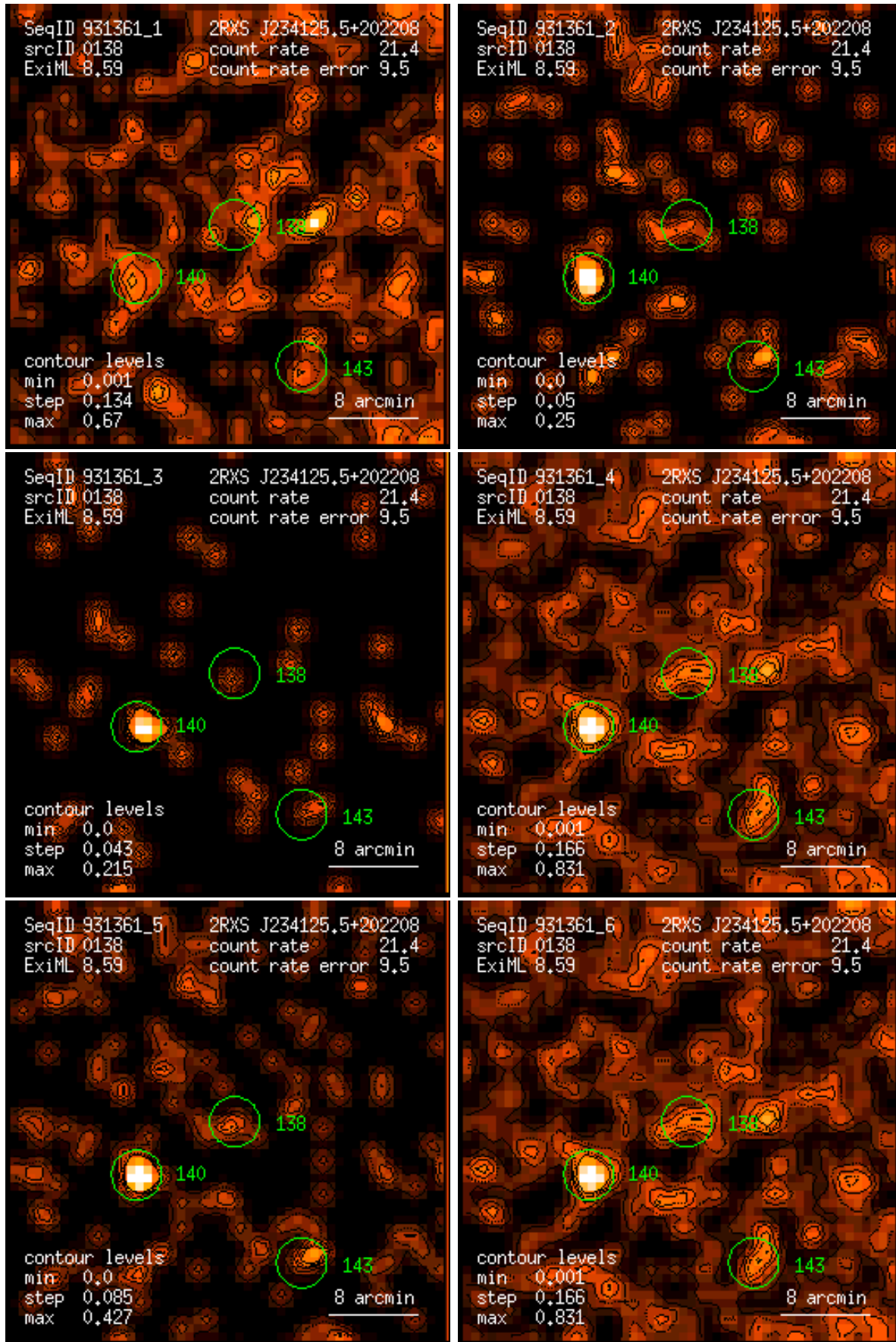
Figure 138: RASS 931361: detection 0138: band rate images, Gaussian filter: (1) PSPC channels 11 – 41, (2) 52 – 90, (3) 91 – 201, (4) 11 – 235, (5) 52 – 201, (6) 11 – 201. Broad band rates in counts/ks. Band rate contour levels in counts/ks/arcmin 2 .
