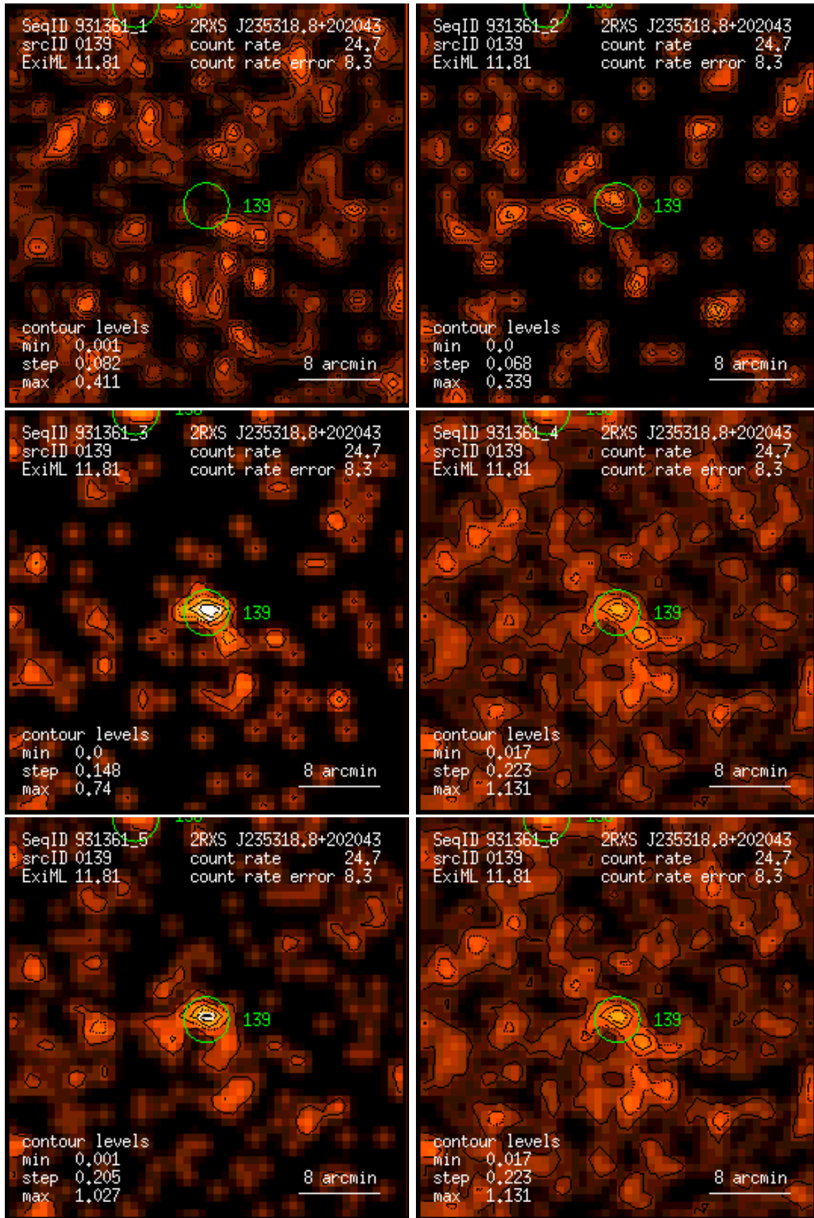
Figure 139: RASS 931361: detection 0139: band rate images, Gaussian filter: (1) PSPC channels 11 – 41, (2) 52 – 90, (3) 91 – 201, (4) 11 – 235, (5) 52 – 201, (6) 11 – 201. Broad band rates in counts/ks. Band rate contour levels in counts/ks/arcmin 2 .
