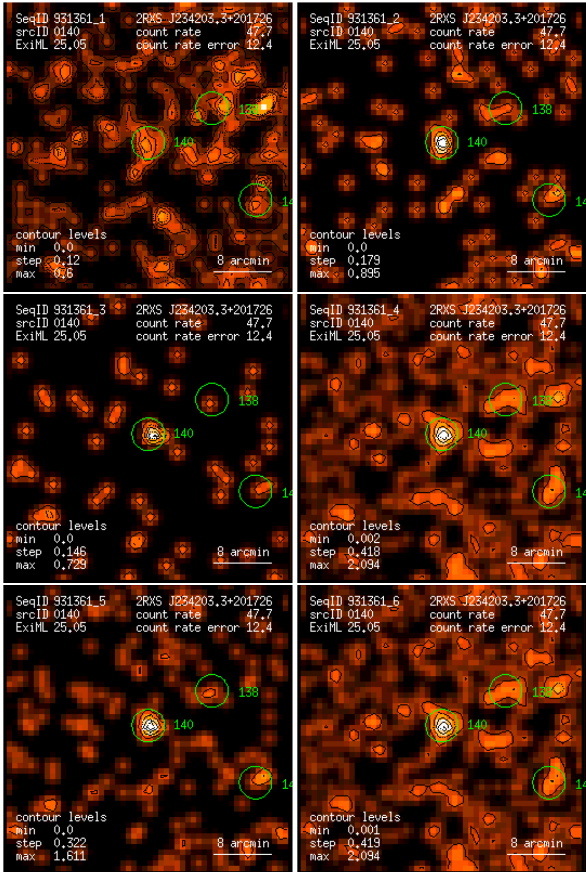
Figure 140: RASS 931361: detection 0140: band rate images, Gaussian filter: (1) PSPC channels 11 – 41, (2) 52 – 90, (3) 91 – 201, (4) 11 – 235, (5) 52 – 201, (6) 11 – 201. Broad band rates in counts/ks. Band rate contour levels in counts/ks/arcmin 2 .
