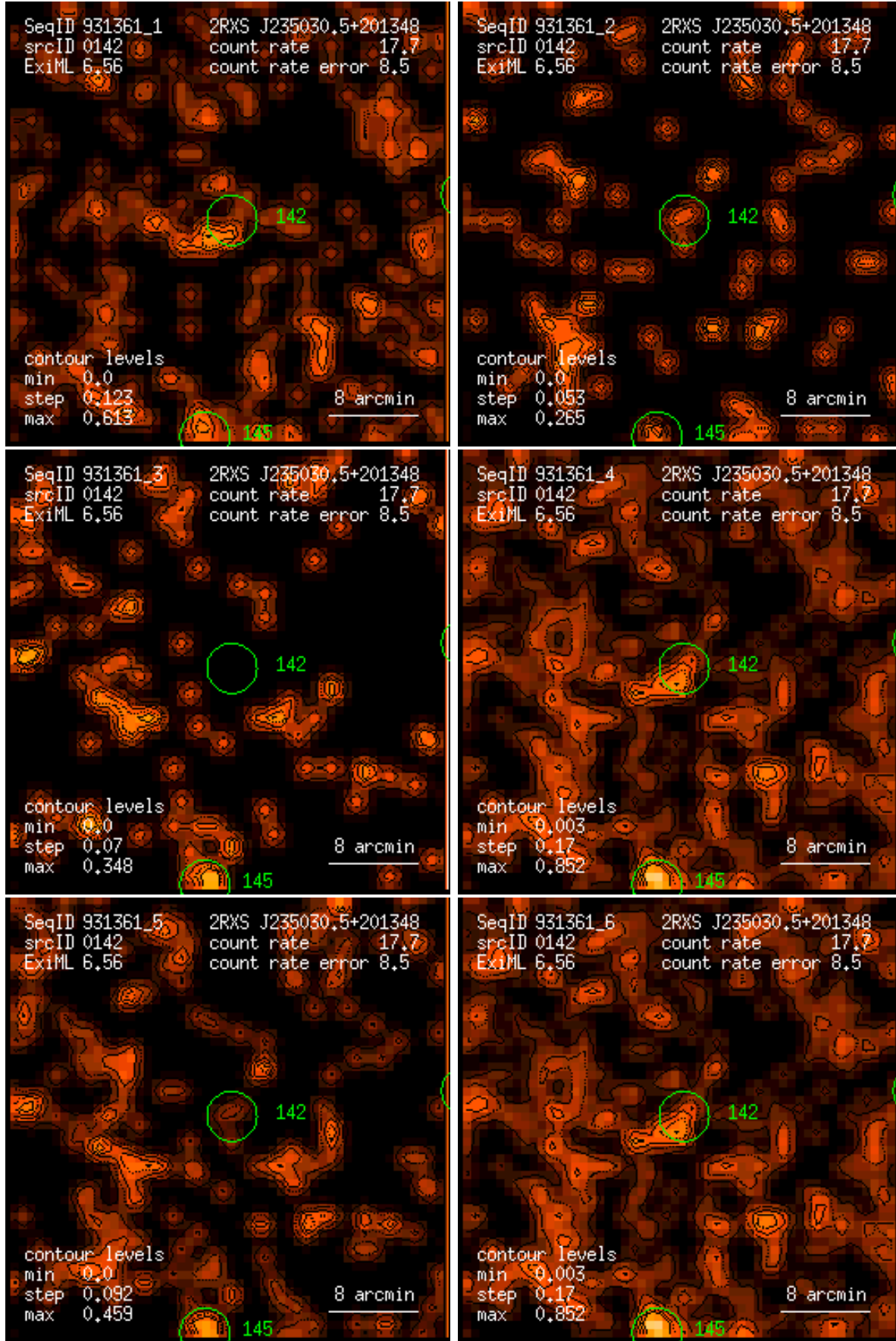
Figure 142: RASS 931361: detection 0142: band rate images, Gaussian filter: (1) PSPC channels 11 – 41, (2) 52 – 90, (3) 91 – 201, (4) 11 – 235, (5) 52 – 201, (6) 11 – 201. Broad band rates in counts/ks. Band rate contour levels in counts/ks/arcmin 2 .
