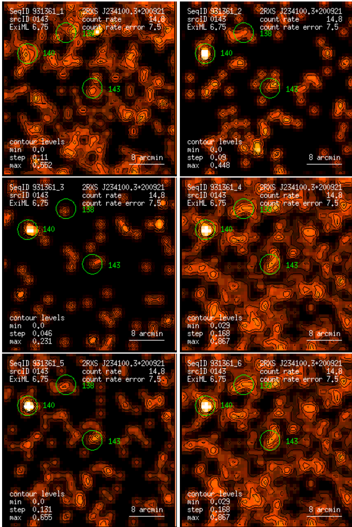
Figure 143: RASS 931361: detection 0143: band rate images, Gaussian filter: (1) PSPC channels 11 – 41, (2) 52 – 90, (3) 91 – 201, (4) 11 – 235, (5) 52 – 201, (6) 11 – 201. Broad band rates in counts/ks. Band rate contour levels in counts/ks/arcmin 2 .
