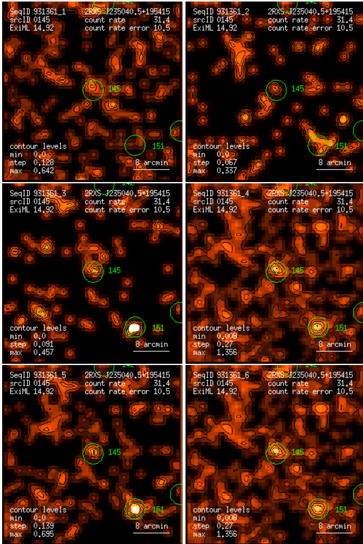
Figure 145: RASS 931361: detection 0145: band rate images, Gaussian filter: (1) PSPC channels 11 – 41, (2) 52 – 90, (3) 91 – 201, (4) 11 – 235, (5) 52 – 201, (6) 11 – 201. Broad band rates in counts/ks. Band rate contour levels in counts/ks/arcmin 2 .
