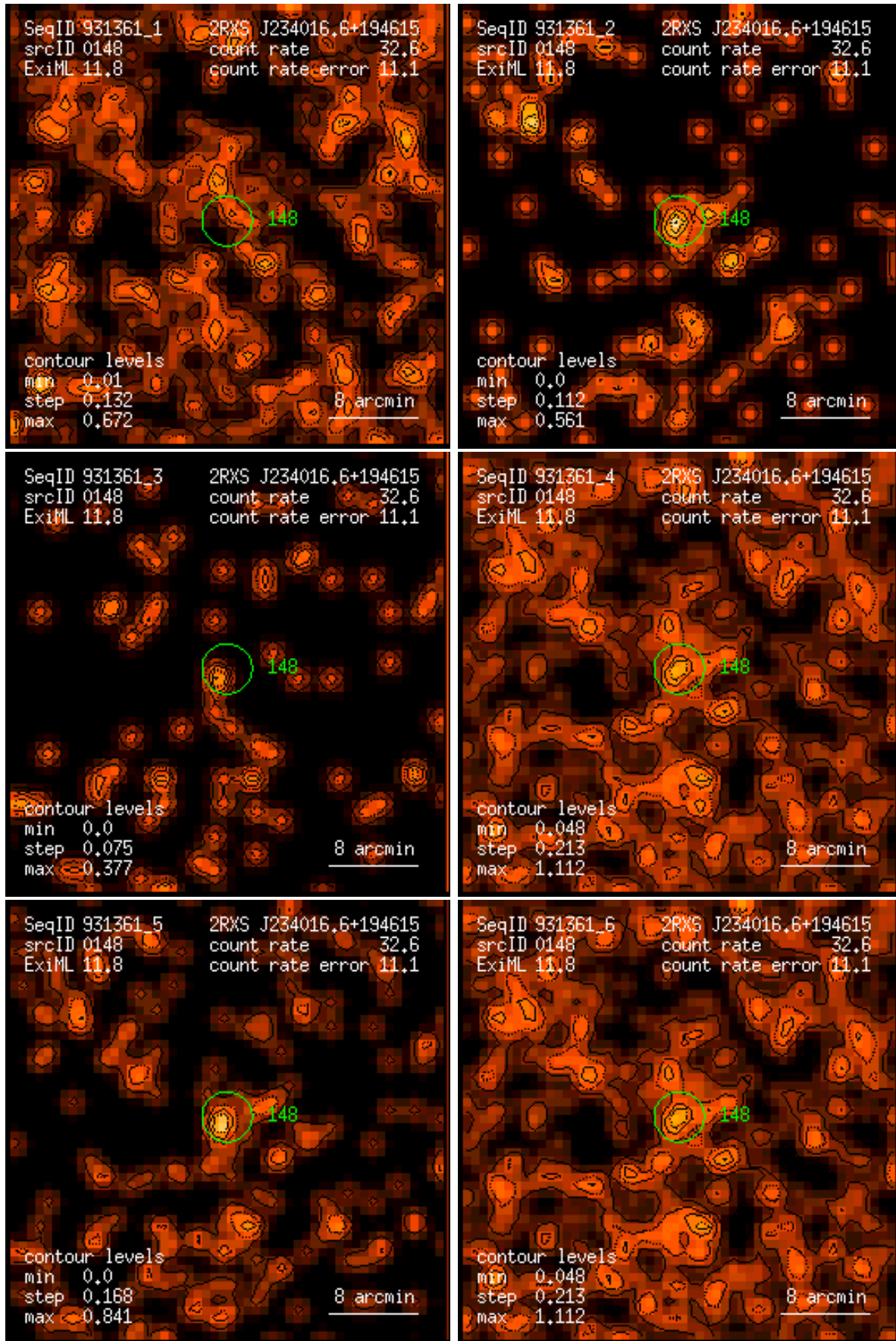
Figure 148: RASS 931361: detection 0148: band rate images, Gaussian filter: (1) PSPC channels 11 – 41, (2) 52 – 90, (3) 91 – 201, (4) 11 – 235, (5) 52 – 201, (6) 11 – 201. Broad band rates in counts/ks. Band rate contour levels in counts/ks/arcmin 2 .
