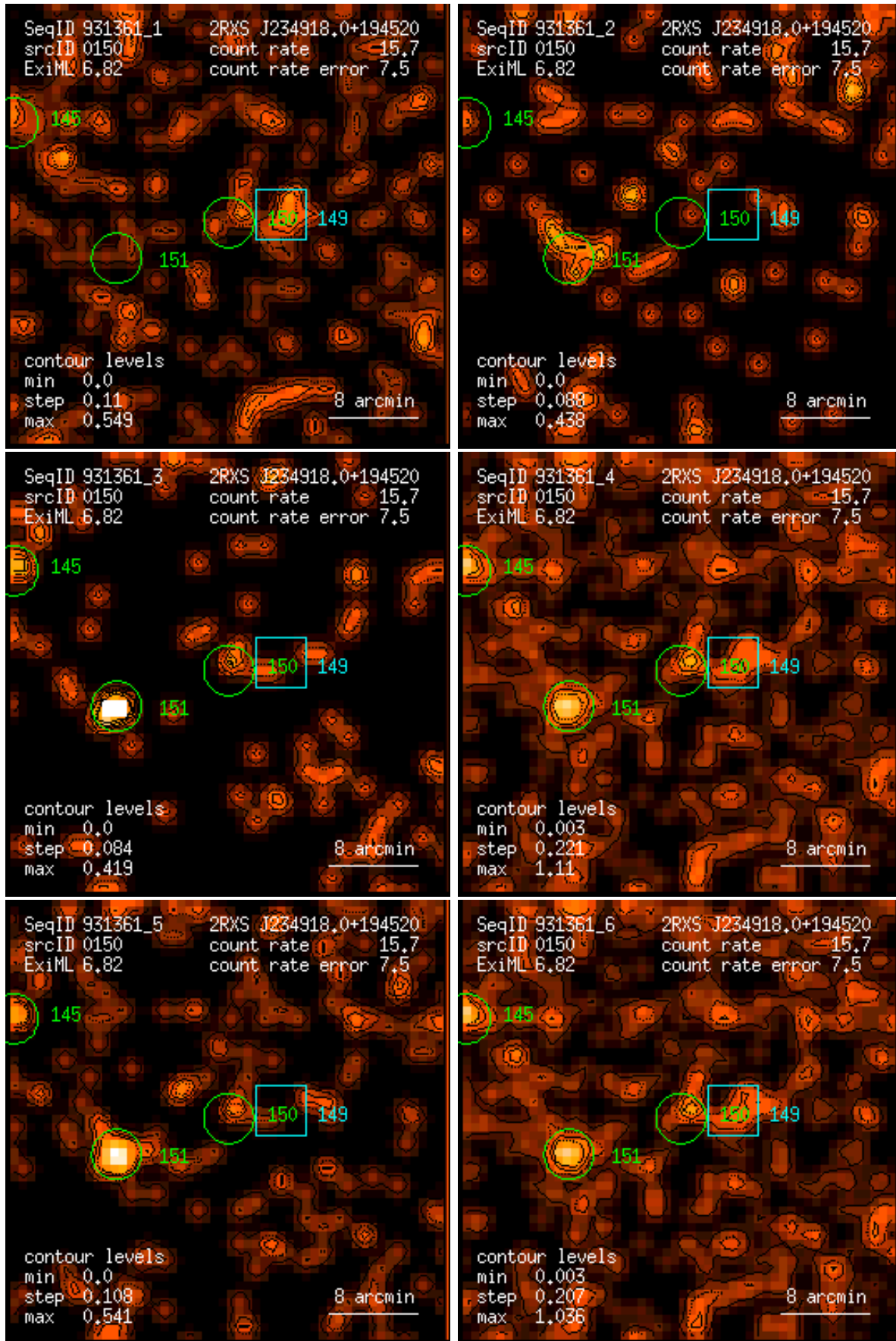
Figure 150: RASS 931361: detection 0150: band rate images, Gaussian filter: (1) PSPC channels 11 – 41, (2) 52 – 90, (3) 91 – 201, (4) 11 – 235, (5) 52 – 201, (6) 11 – 201. Broad band rates in counts/ks. Band rate contour levels in counts/ks/arcmin 2 .
