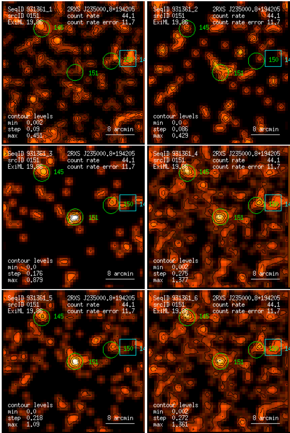
Figure 151: RASS 931361: detection 0151: band rate images, Gaussian filter: (1) PSPC channels 11 – 41, (2) 52 – 90, (3) 91 – 201, (4) 11 – 235, (5) 52 – 201, (6) 11 – 201. Broad band rates in counts/ks. Band rate contour levels in counts/ks/arcmin 2 .
