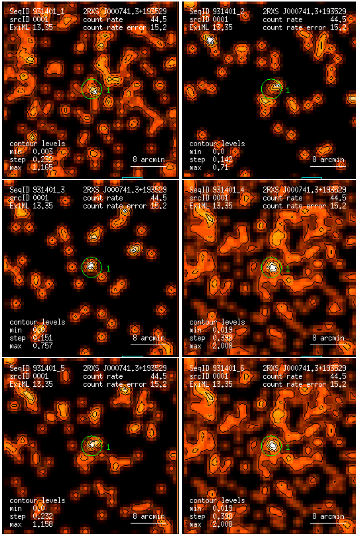
Figure 1: RASS 931401: detection 0001: band rate images, Gaussian filter: (1) PSPC channels 11 – 41, (2) 52 – 90, (3) 91 – 201, (4) 11 – 235, (5) 52 – 201, (6) 11 – 201. Broad band rates in counts/ks. Band rate contour levels in counts/ks/arcmin 2 .
