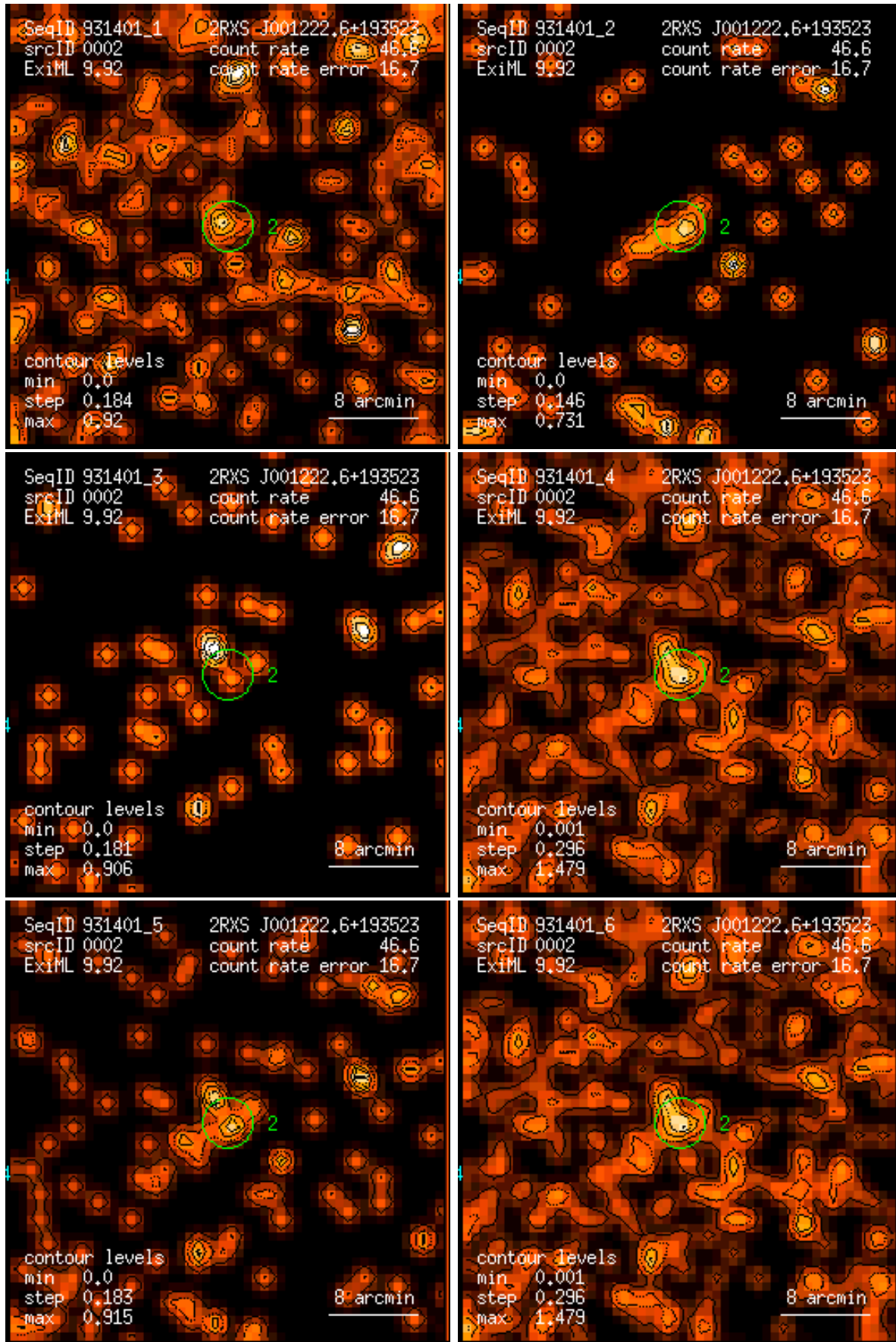
Figure 2: RASS 931401: detection 0002: band rate images, Gaussian filter: (1) PSPC channels 11 – 41, (2) 52 – 90, (3) 91 – 201, (4) 11 – 235, (5) 52 – 201, (6) 11 – 201. Broad band rates in counts/ks. Band rate contour levels in counts/ks/arcmin 2 .
