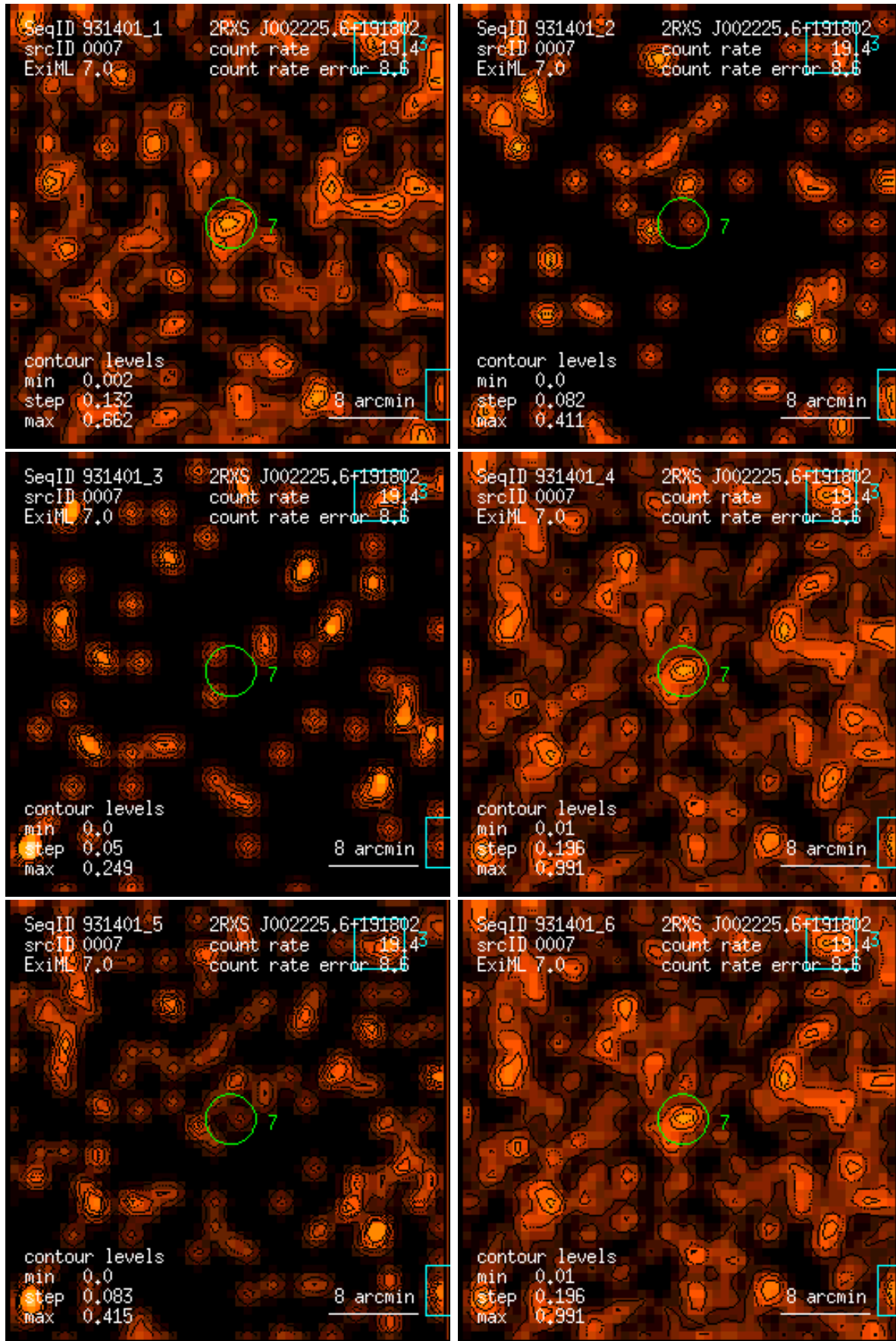
Figure 7: RASS 931401: detection 0007: band rate images, Gaussian filter: (1) PSPC channels 11 – 41, (2) 52 – 90, (3) 91 – 201, (4) 11 – 235, (5) 52 – 201, (6) 11 – 201. Broad band rates in counts/ks. Band rate contour levels in counts/ks/arcmin 2 .
