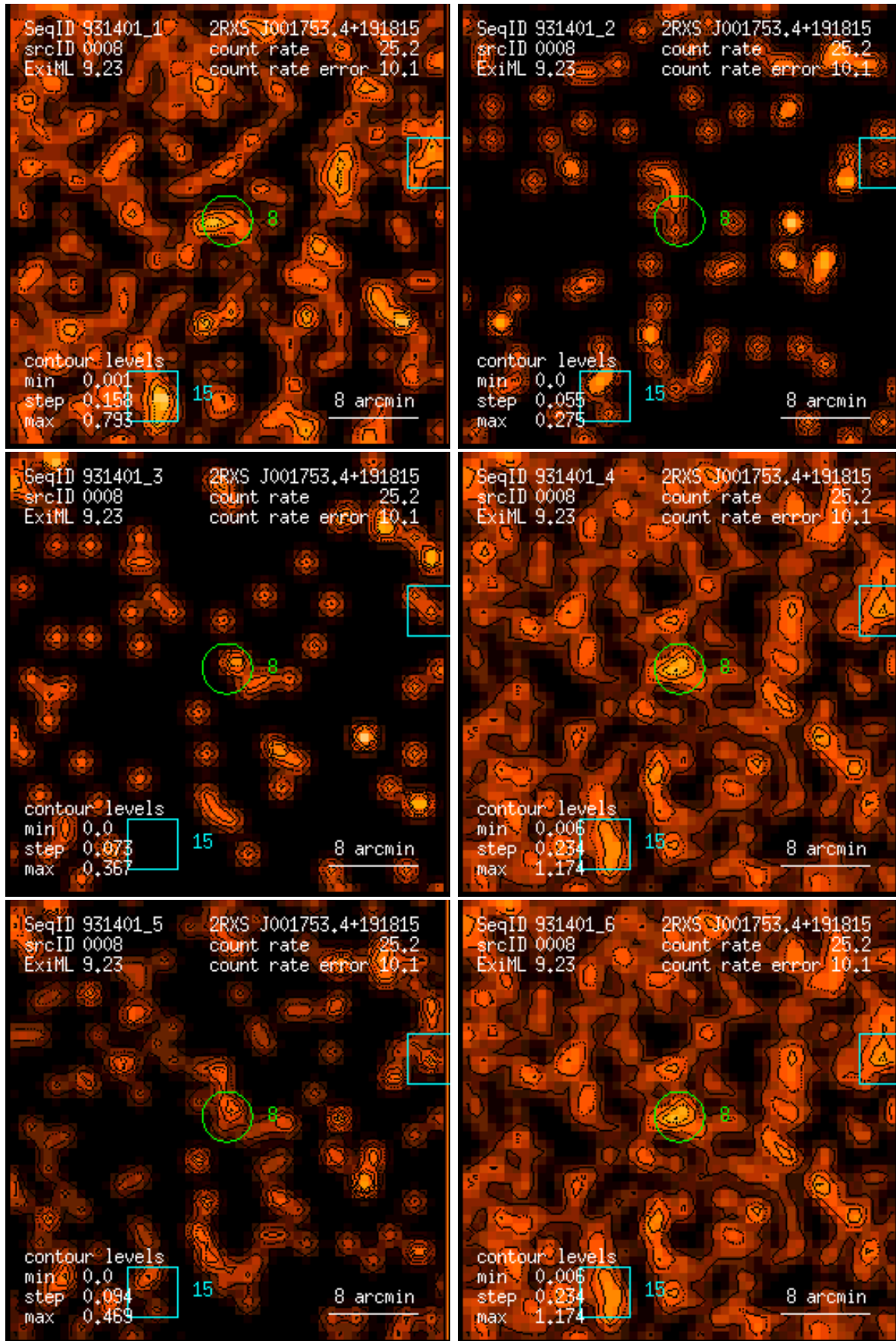
Figure 8: RASS 931401: detection 0008: band rate images, Gaussian filter: (1) PSPC channels 11 – 41, (2) 52 – 90, (3) 91 – 201, (4) 11 – 235, (5) 52 – 201, (6) 11 – 201. Broad band rates in counts/ks. Band rate contour levels in counts/ks/arcmin 2 .
