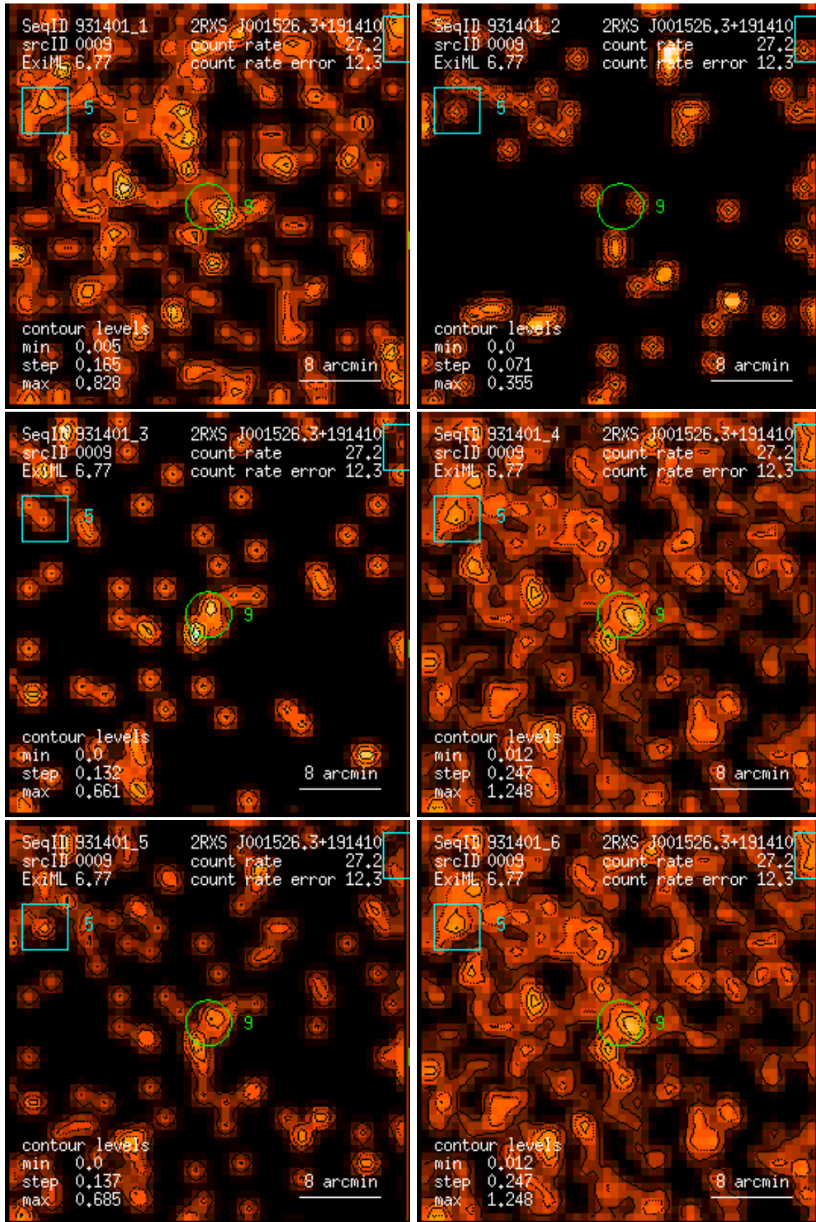
Figure 9: RASS 931401: detection 0009: band rate images, Gaussian filter: (1) PSPC channels 11 – 41, (2) 52 – 90, (3) 91 – 201, (4) 11 – 235, (5) 52 – 201, (6) 11 – 201. Broad band rates in counts/ks. Band rate contour levels in counts/ks/arcmin 2 .
