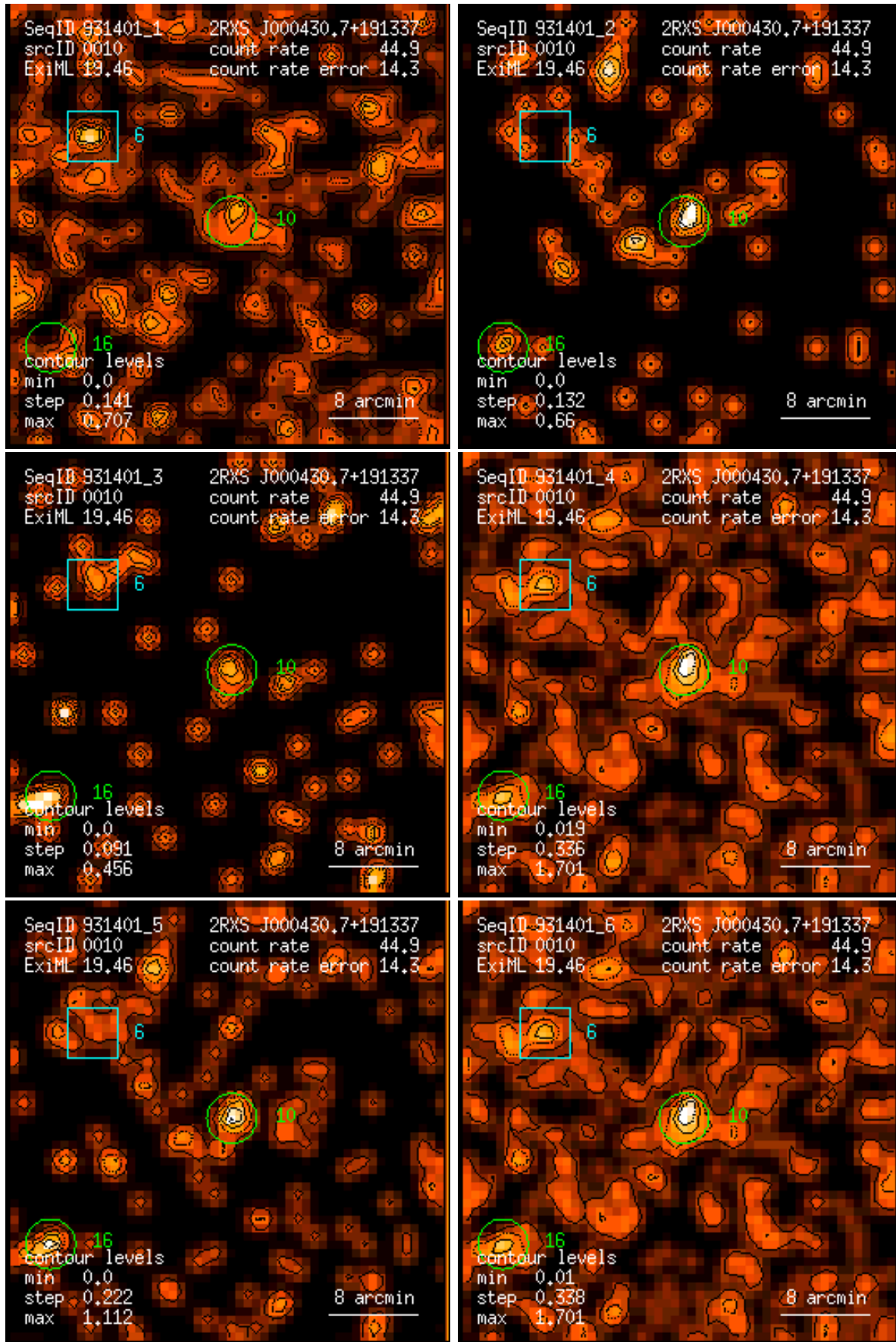
Figure 10: RASS 931401: detection 0010: band rate images, Gaussian filter: (1) PSPC channels 11 – 41, (2) 52 – 90, (3) 91 – 201, (4) 11 – 235, (5) 52 – 201, (6) 11 – 201. Broad band rates in counts/ks. Band rate contour levels in counts/ks/arcmin 2 .
