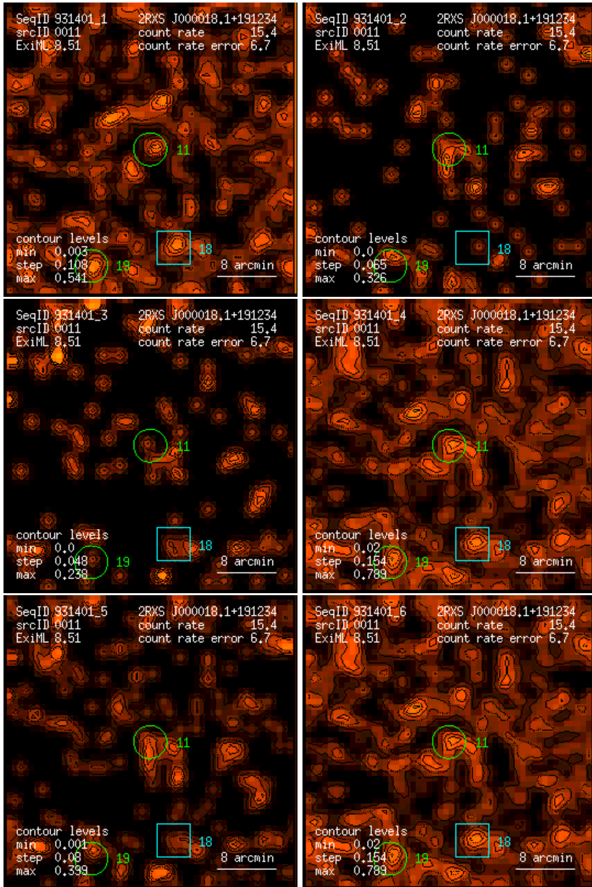
Figure 11: RASS 931401: detection 0011: band rate images, Gaussian filter: (1) PSPC channels 11 – 41, (2) 52 – 90, (3) 91 – 201, (4) 11 – 235, (5) 52 – 201, (6) 11 – 201. Broad band rates in counts/ks. Band rate contour levels in counts/ks/arcmin 2 .
