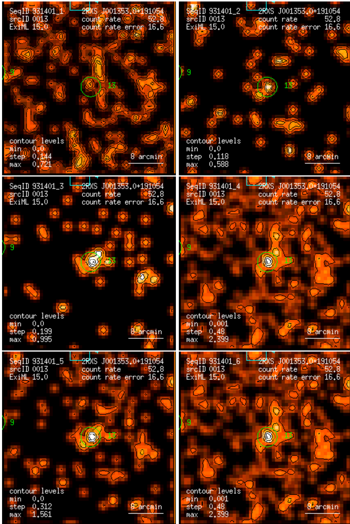
Figure 13: RASS 931401: detection 0013: band rate images, Gaussian filter: (1) PSPC channels 11 – 41, (2) 52 – 90, (3) 91 – 201, (4) 11 – 235, (5) 52 – 201, (6) 11 – 201. Broad band rates in counts/ks. Band rate contour levels in counts/ks/arcmin 2 .
