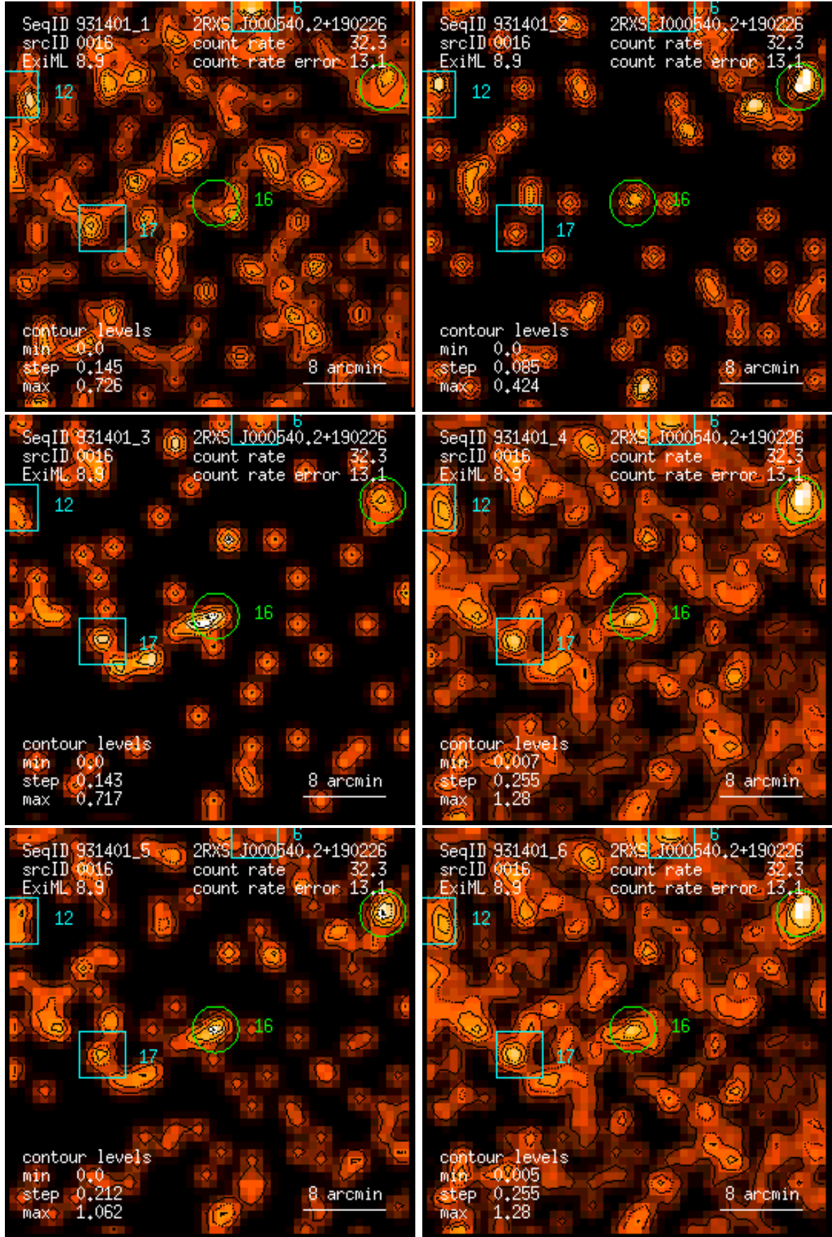
Figure 16: RASS 931401: detection 0016: band rate images, Gaussian filter: (1) PSPC channels 11 – 41, (2) 52 – 90, (3) 91 – 201, (4) 11 – 235, (5) 52 – 201, (6) 11 – 201. Broad band rates in counts/ks. Band rate contour levels in counts/ks/arcmin 2 .
