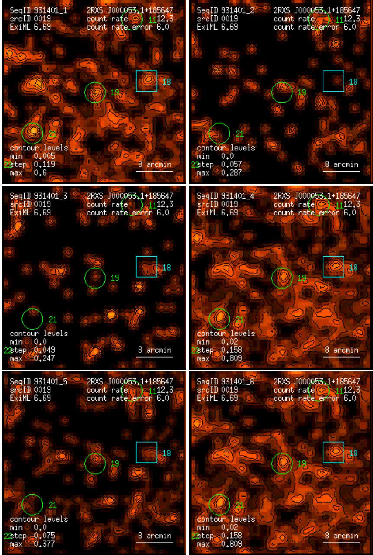
Figure 19: RASS 931401: detection 0019: band rate images, Gaussian filter: (1) PSPC channels 11 – 41, (2) 52 – 90, (3) 91 – 201, (4) 11 – 235, (5) 52 – 201, (6) 11 – 201. Broad band rates in counts/ks. Band rate contour levels in counts/ks/arcmin 2 .
