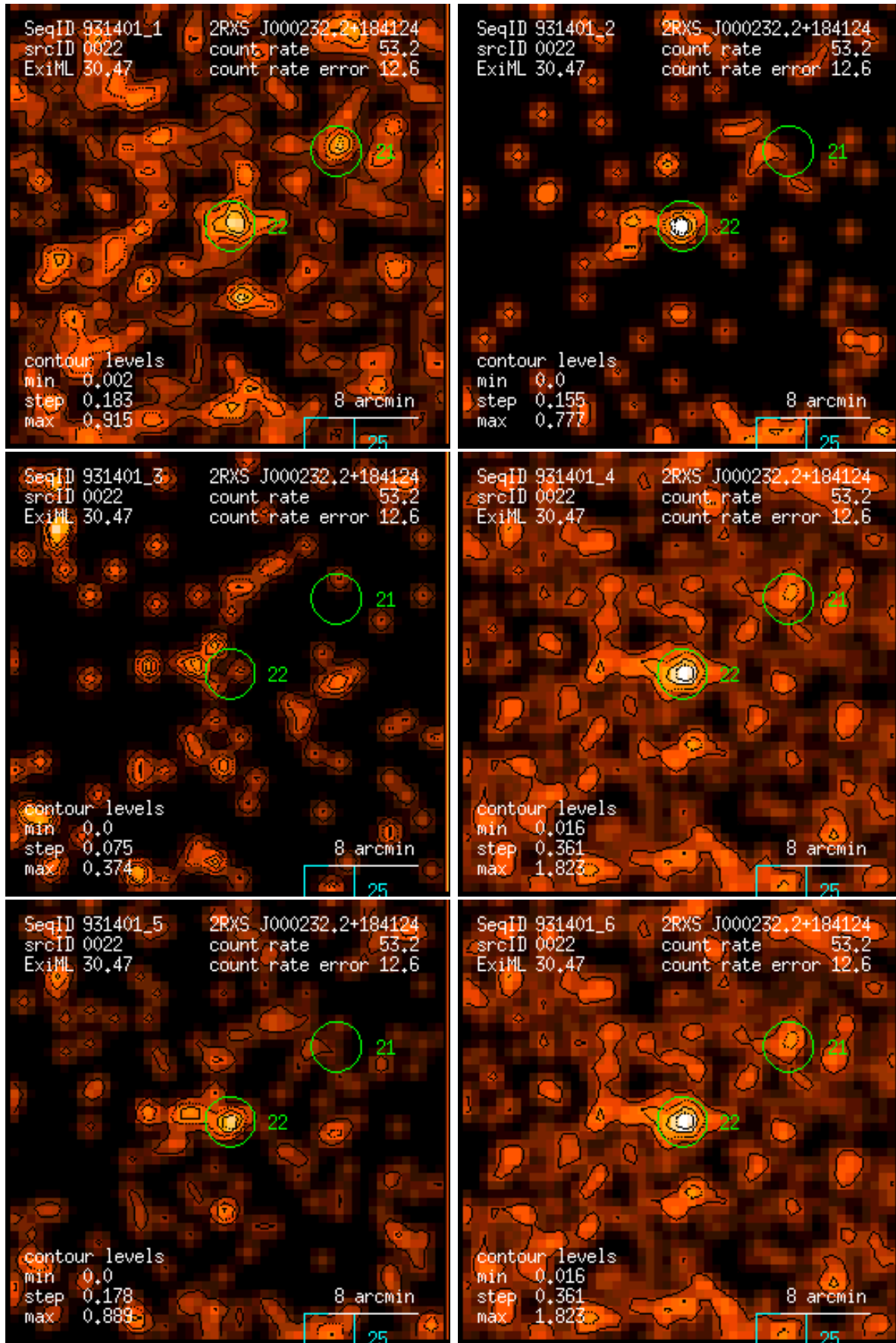
Figure 22: RASS 931401: detection 0022: band rate images, Gaussian filter: (1) PSPC channels 11 – 41, (2) 52 – 90, (3) 91 – 201, (4) 11 – 235, (5) 52 – 201, (6) 11 – 201. Broad band rates in counts/ks. Band rate contour levels in counts/ks/arcmin 2 .
