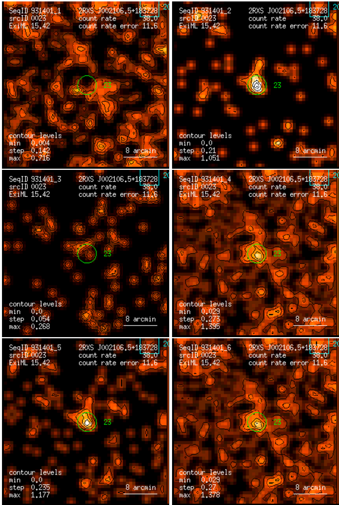
Figure 23: RASS 931401: detection 0023: band rate images, Gaussian filter: (1) PSPC channels 11 – 41, (2) 52 – 90, (3) 91 – 201, (4) 11 – 235, (5) 52 – 201, (6) 11 – 201. Broad band rates in counts/ks. Band rate contour levels in counts/ks/arcmin 2 .
