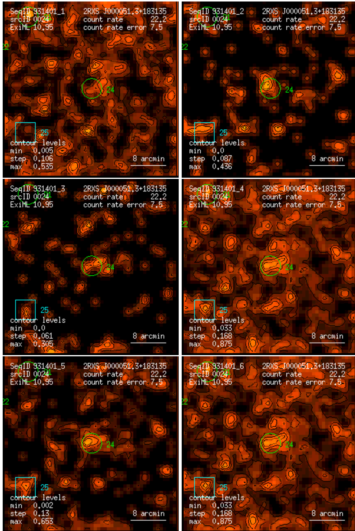
Figure 24: RASS 931401: detection 0024: band rate images, Gaussian filter: (1) PSPC channels 11 – 41, (2) 52 – 90, (3) 91 – 201, (4) 11 – 235, (5) 52 – 201, (6) 11 – 201. Broad band rates in counts/ks. Band rate contour levels in counts/ks/arcmin 2 .
