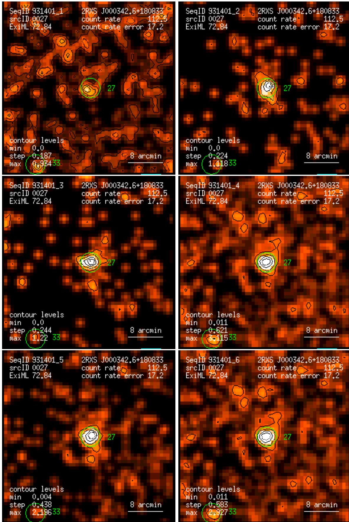
Figure 27: RASS 931401: detection 0027: band rate images, Gaussian filter: (1) PSPC channels 11 – 41, (2) 52 – 90, (3) 91 – 201, (4) 11 – 235, (5) 52 – 201, (6) 11 – 201. Broad band rates in counts/ks. Band rate contour levels in counts/ks/arcmin 2 .
