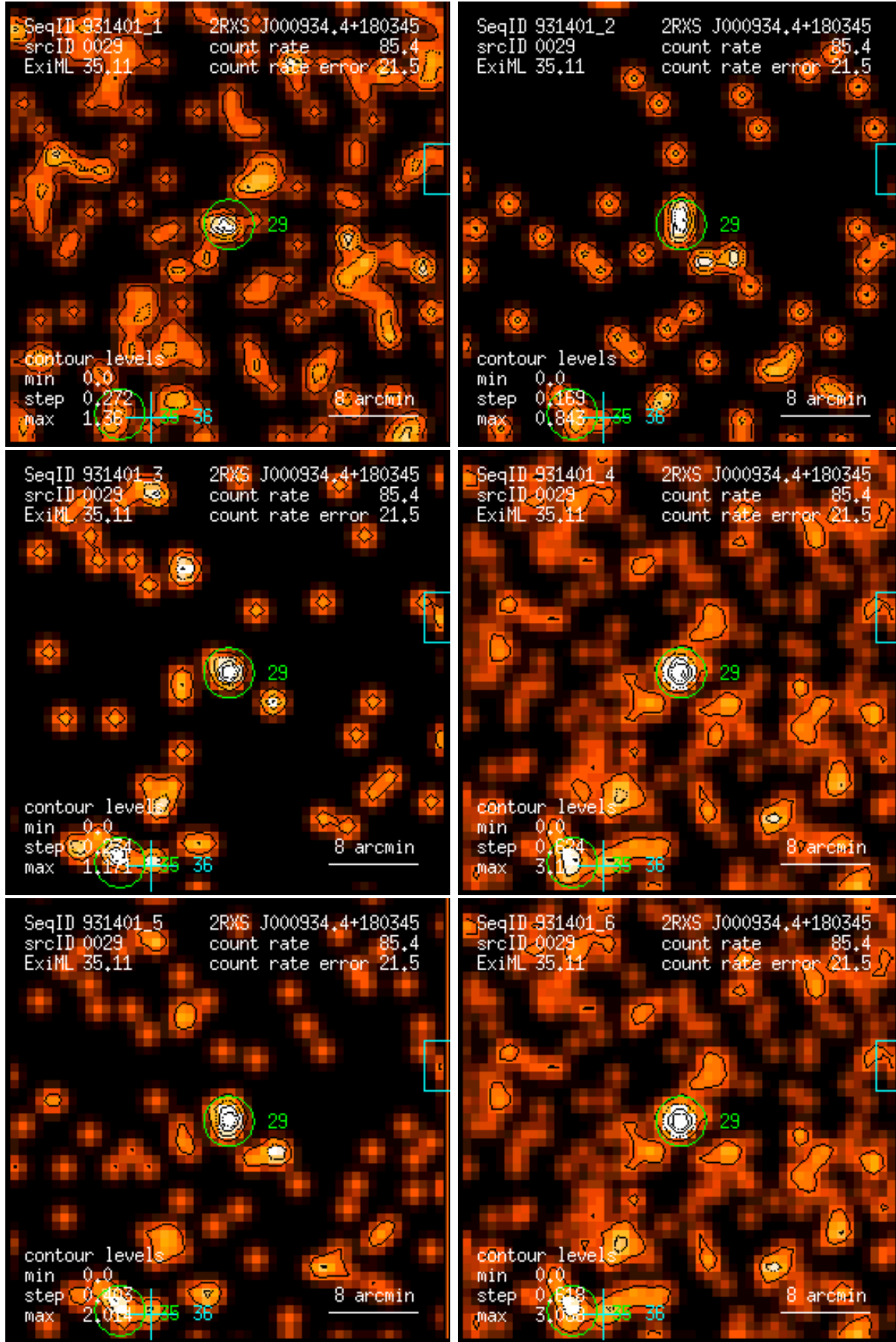
Figure 29: RASS 931401: detection 0029: band rate images, Gaussian filter: (1) PSPC channels 11 – 41, (2) 52 – 90, (3) 91 – 201, (4) 11 – 235, (5) 52 – 201, (6) 11 – 201. Broad band rates in counts/ks. Band rate contour levels in counts/ks/arcmin 2 .
