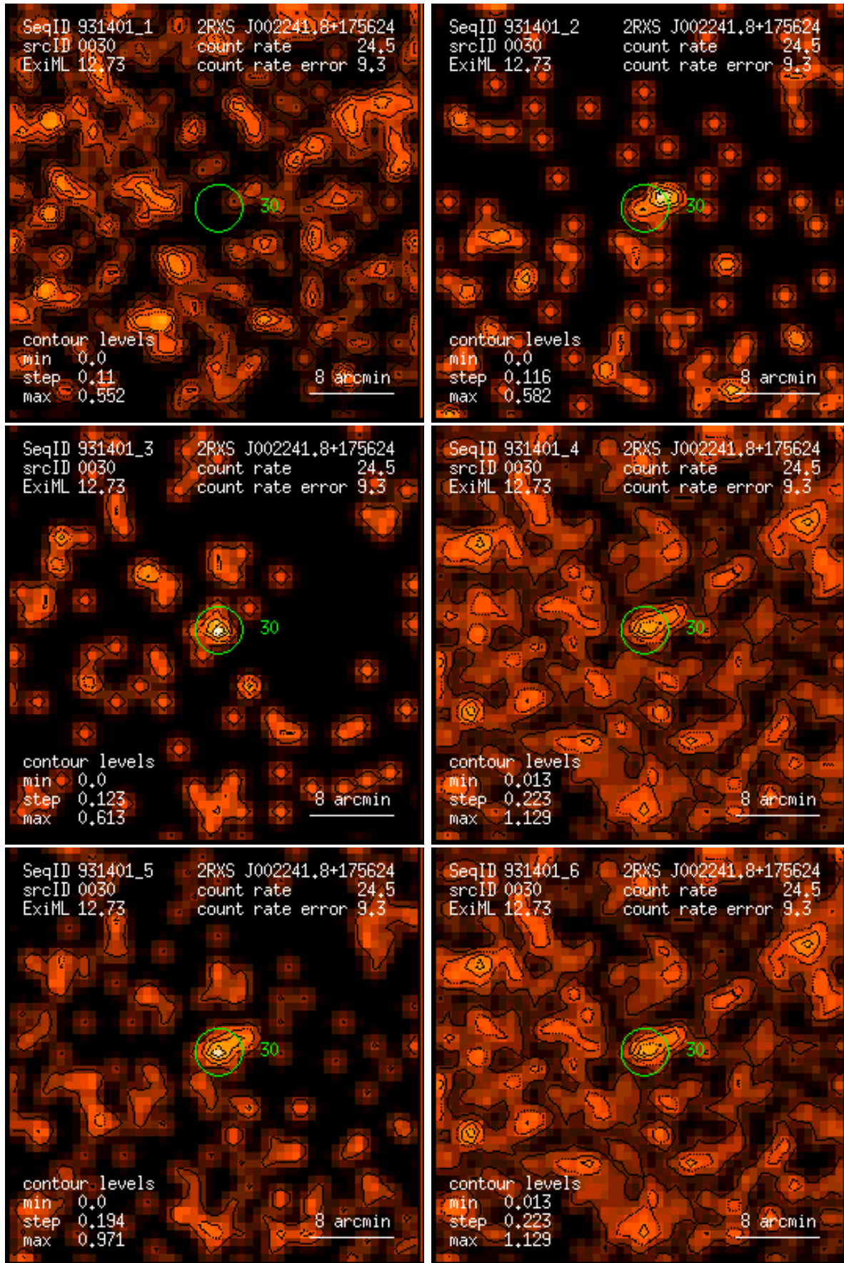
Figure 30: RASS 931401: detection 0030: band rate images, Gaussian filter: (1) PSPC channels 11 – 41, (2) 52 – 90, (3) 91 – 201, (4) 11 – 235, (5) 52 – 201, (6) 11 – 201. Broad band rates in counts/ks. Band rate contour levels in counts/ks/arcmin 2 .
