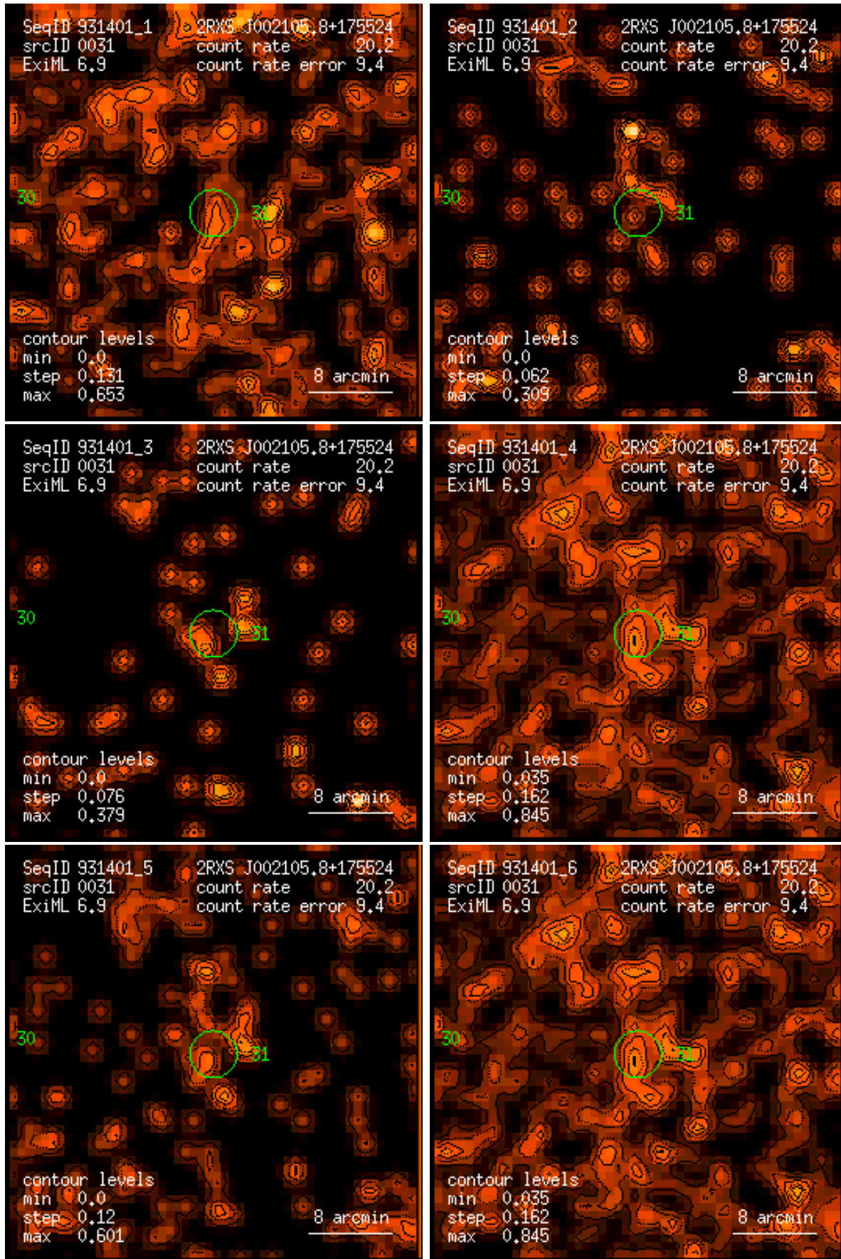
Figure 31: RASS 931401: detection 0031: band rate images, Gaussian filter: (1) PSPC channels 11 – 41, (2) 52 – 90, (3) 91 – 201, (4) 11 – 235, (5) 52 – 201, (6) 11 – 201. Broad band rates in counts/ks. Band rate contour levels in counts/ks/arcmin 2 .
