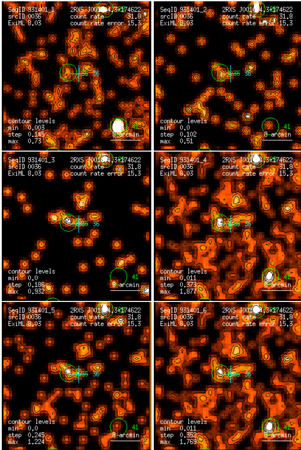
Figure 36: RASS 931401: detection 0036: band rate images, Gaussian filter: (1) PSPC channels 11 – 41, (2) 52 – 90, (3) 91 – 201, (4) 11 – 235, (5) 52 – 201, (6) 11 – 201. Broad band rates in counts/ks. Band rate contour levels in counts/ks/arcmin 2 .
