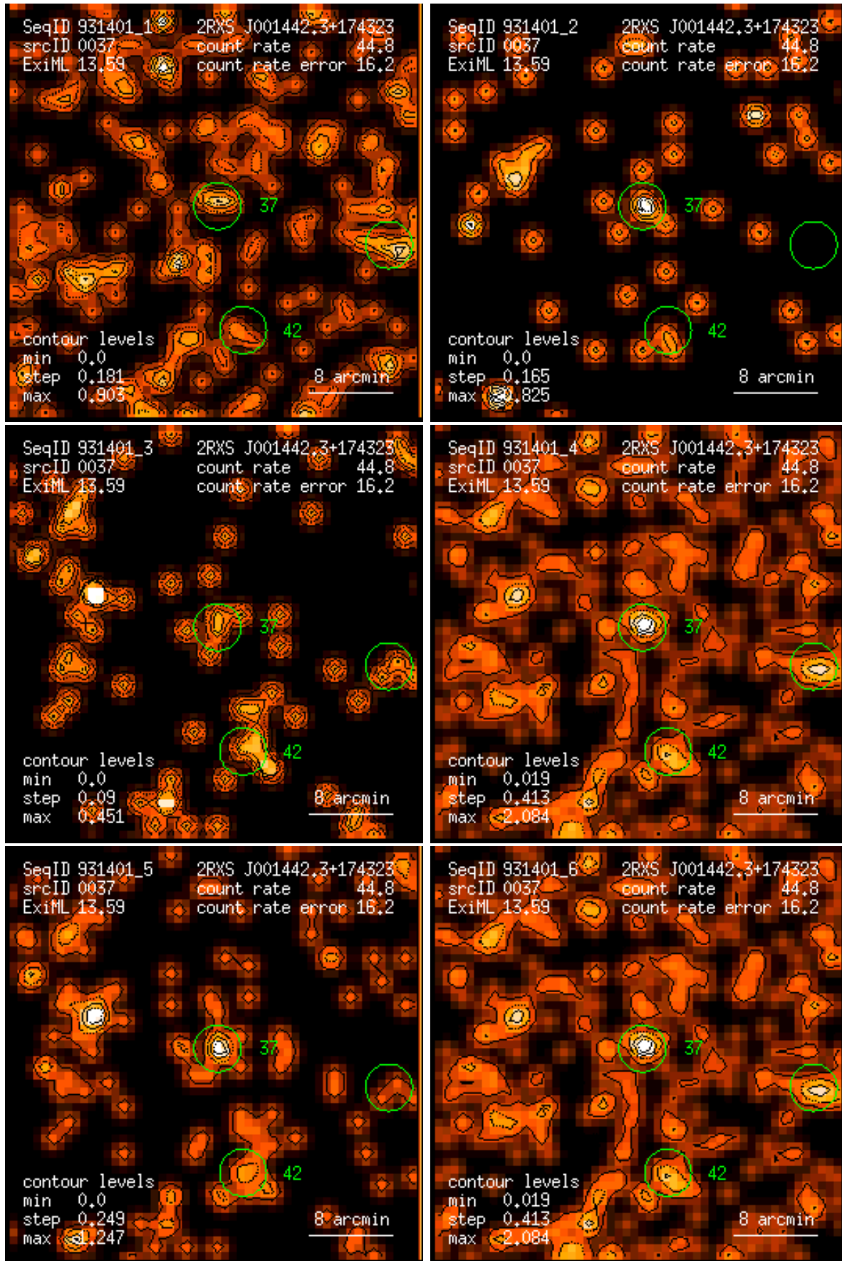
Figure 37: RASS 931401: detection 0037: band rate images, Gaussian filter: (1) PSPC channels 11 – 41, (2) 52 – 90, (3) 91 – 201, (4) 11 – 235, (5) 52 – 201, (6) 11 – 201. Broad band rates in counts/ks. Band rate contour levels in counts/ks/arcmin 2 .
