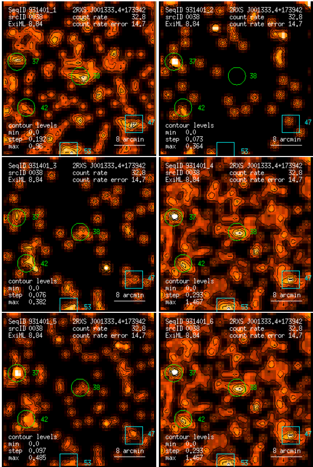
Figure 38: RASS 931401: detection 0038: band rate images, Gaussian filter: (1) PSPC channels 11 – 41, (2) 52 – 90, (3) 91 – 201, (4) 11 – 235, (5) 52 – 201, (6) 11 – 201. Broad band rates in counts/ks. Band rate contour levels in counts/ks/arcmin 2 .
