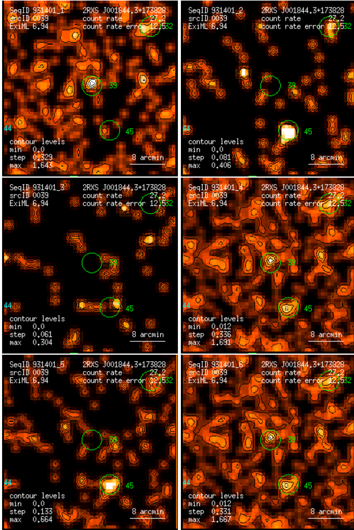
Figure 39: RASS 931401: detection 0039: band rate images, Gaussian filter: (1) PSPC channels 11 – 41, (2) 52 – 90, (3) 91 – 201, (4) 11 – 235, (5) 52 – 201, (6) 11 – 201. Broad band rates in counts/ks. Band rate contour levels in counts/ks/arcmin 2 .
