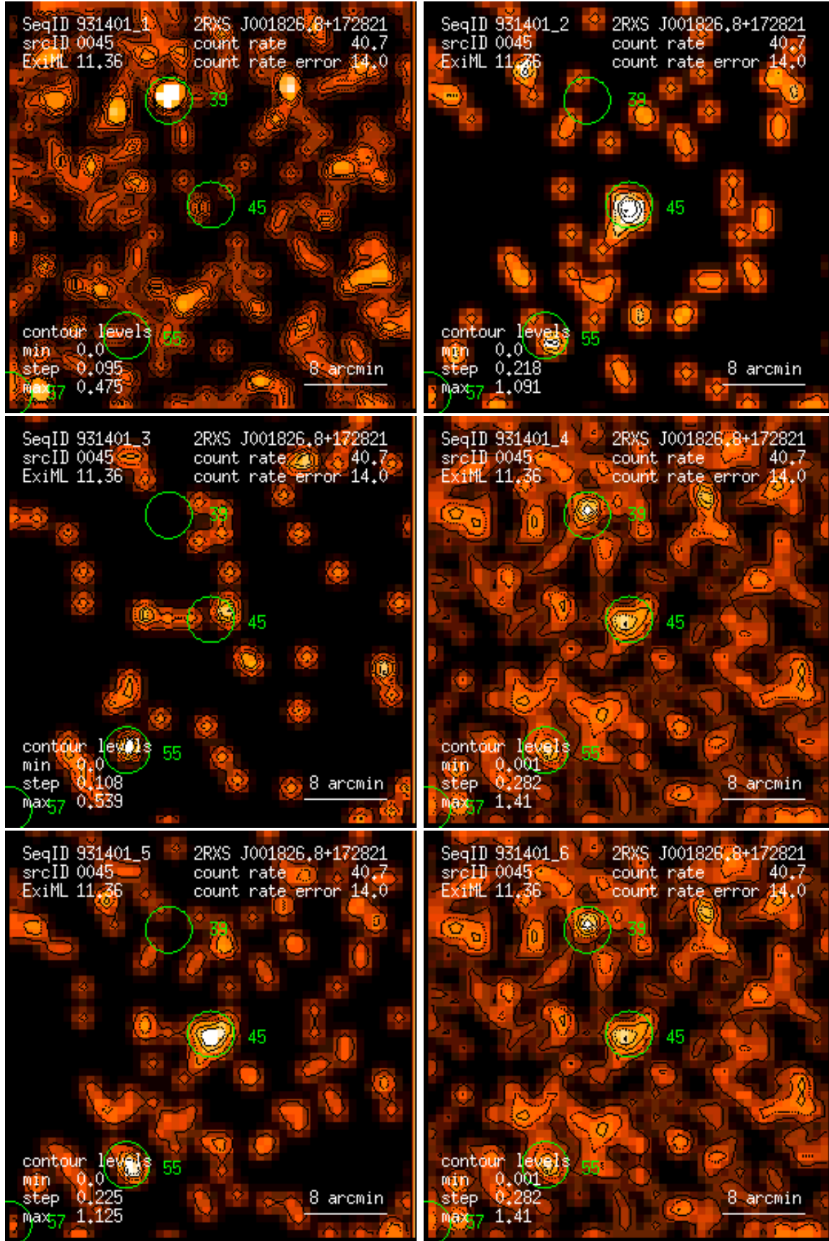
Figure 45: RASS 931401: detection 0045: band rate images, Gaussian filter: (1) PSPC channels 11 – 41, (2) 52 – 90, (3) 91 – 201, (4) 11 – 235, (5) 52 – 201, (6) 11 – 201. Broad band rates in counts/ks. Band rate contour levels in counts/ks/arcmin 2 .
