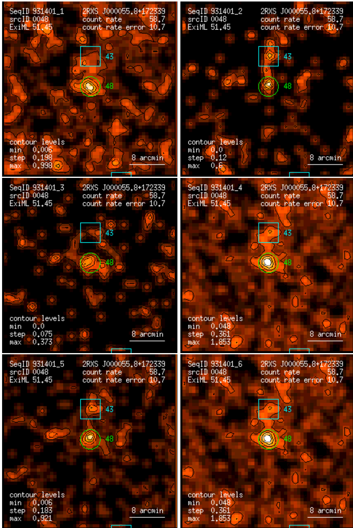
Figure 48: RASS 931401: detection 0048: band rate images, Gaussian filter: (1) PSPC channels 11 – 41, (2) 52 – 90, (3) 91 – 201, (4) 11 – 235, (5) 52 – 201, (6) 11 – 201. Broad band rates in counts/ks. Band rate contour levels in counts/ks/arcmin 2 .
